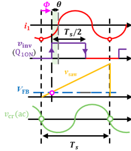
(b) Timing chart of D-EPC
