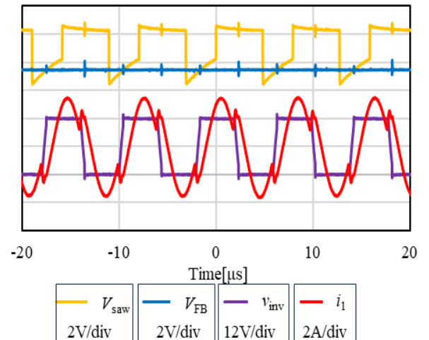
Fig.11. Operating wave form
