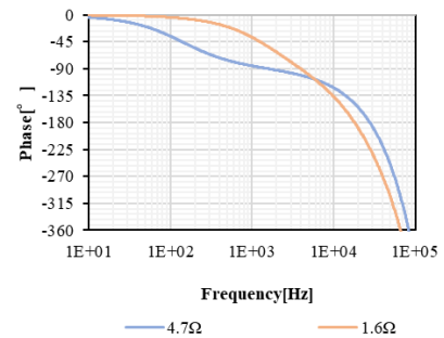
(b) Phase characteristics
