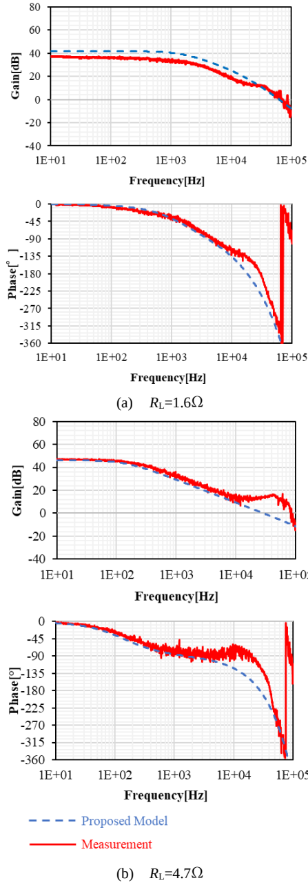
Fig.12. Experimental result (control to output bode plot)
