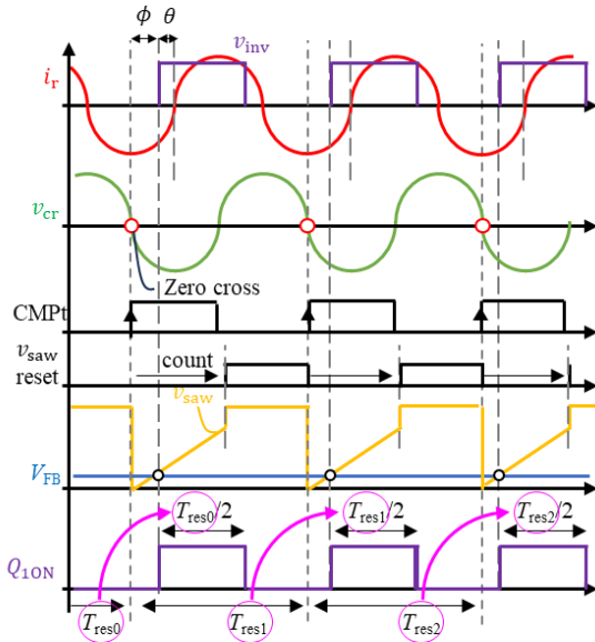
Fig.9. Timing chart of LLC D-EPC
