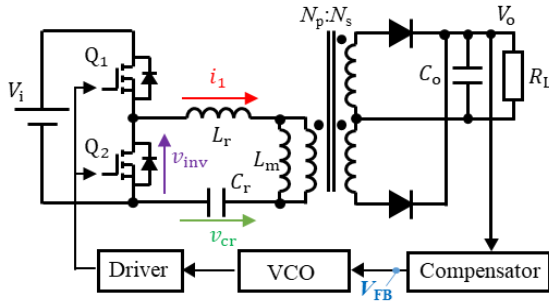
Fig.1. Block diagram of LLC using VCO
