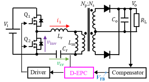
(a) Block diagram of LLC using D-EPC
