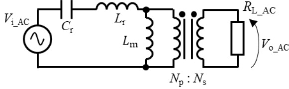
Fig.2. Equivalent circuit of LLC converter using FHA.
