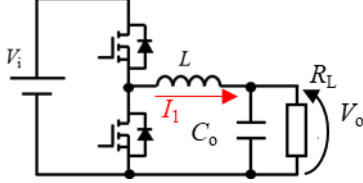
Fig.6. Buck converter
