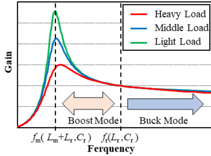
Fig.3. Frequency vs gain characteristic LLC
