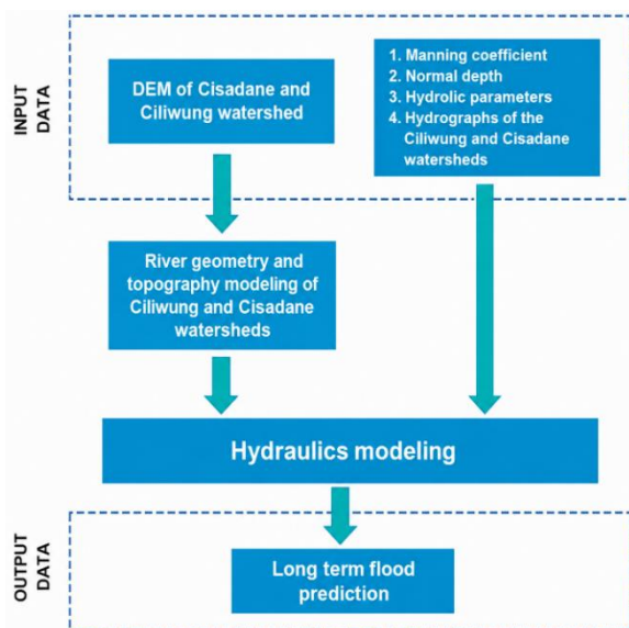
Fig. 4: HEC-RAS Flowchart
