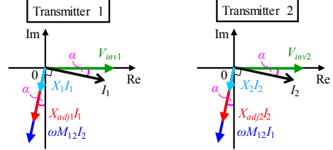
Fig. 5. Phasor diagrams of each transmitter in Fig. 4.
