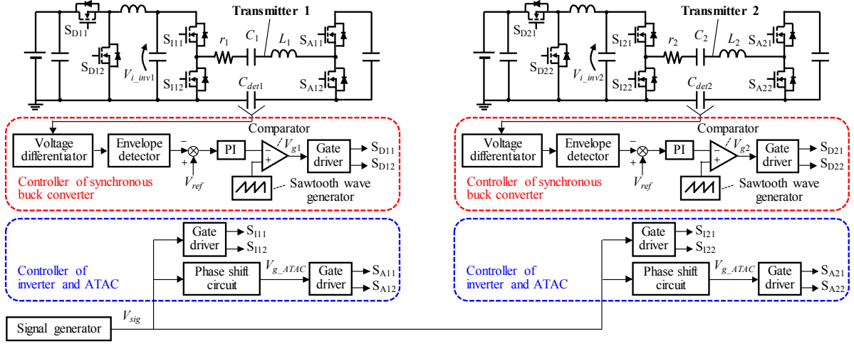
Fig. 8. Practical circuit configuration including controllers of each transmitter.
