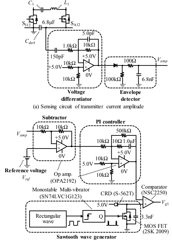
Fig. 9. Controller of synchronous buck converter.
