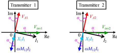
Fig. 7. Phasor diagrams of each transmitter in Fig. 6.
