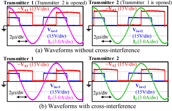
Fig. 15. Experimental waveforms with ATAC.
