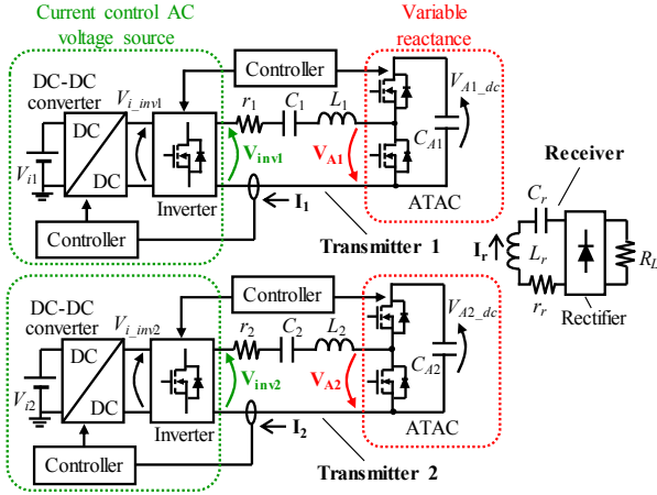
Fig. 6. System configuration of proposed multiple-transmitter RIC-WPT system.
