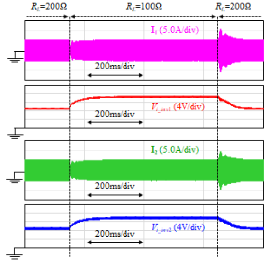
Fig. 13. Experimental results of load variation.
