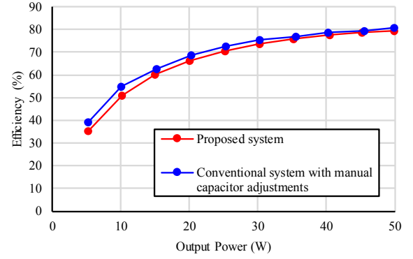
Fig. 16. Comparison of overall efficiencies in RIC-WPT system.
