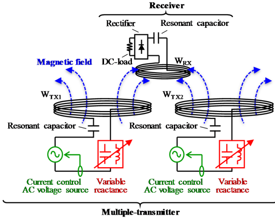
Fig. 3. Concept diagram of proposed multiple-transmitter RIC-WPT system.
