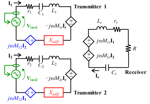
Fig. 4. Equivalent circuit of Fig. 3.
