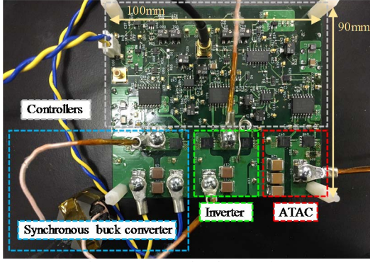
Fig. 12. PCB of each transmitter.
