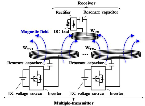
Fig. 2. Typical multiple-transmitter RIC-WPT system.
