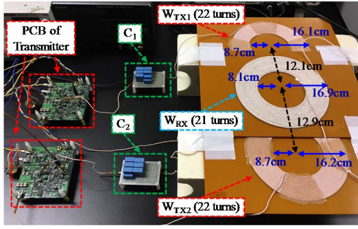
Fig. 11 Experimental setup.
