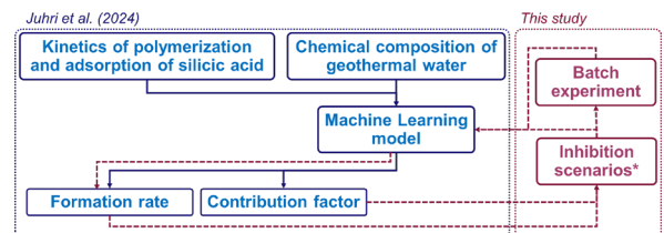
Figure 4: Workflow of the use of machine learning for the prediction of silica scale formation based on several inhibition scenarios.
