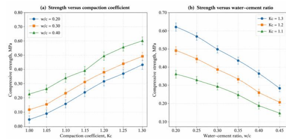
Fig. 2: Effects of compaction coefficient and water-to-cement ratio on RHLC compressive strength
