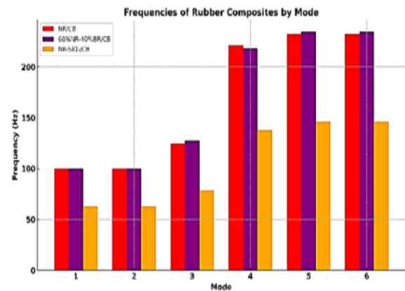
Fig. 22: Maximal Deformation Values for Higher Vibration Modes for Rubber-Based Composites
