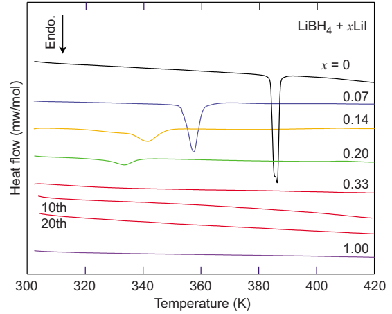
FIG. 2. (Color online) DSC profiles of \text{LiBH}_4 + x\text{LiI} . The intensities are normalized to show the heat flow per mole of the formula unit of \text{LiBH}_4 + x\text{LiI} . The area of the endothermic peak of each profile gives the experimental value of the enthalpy change ( \Delta H_{\text{exp}} ), e.g., 4.18 kJ/mol with x=0 .
