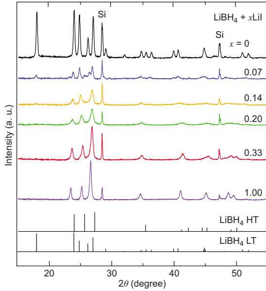
FIG. 1. (Color online) Powder XRD profiles of \text{LiBH}_4 + x\text{LiI} ( x=0-1.00 ). The diffraction peaks are calibrated by Si internal standard. The standard diffraction peaks of the LT (orthorhombic) and HT (hexagonal) phases of \text{LiBH}_4 are shown for reference (Ref. 7).
