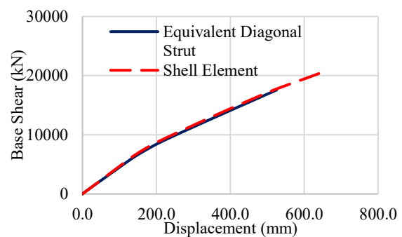
Fig. 14: Y-Axis Capacity Curve of Infilled Frame with Openings
