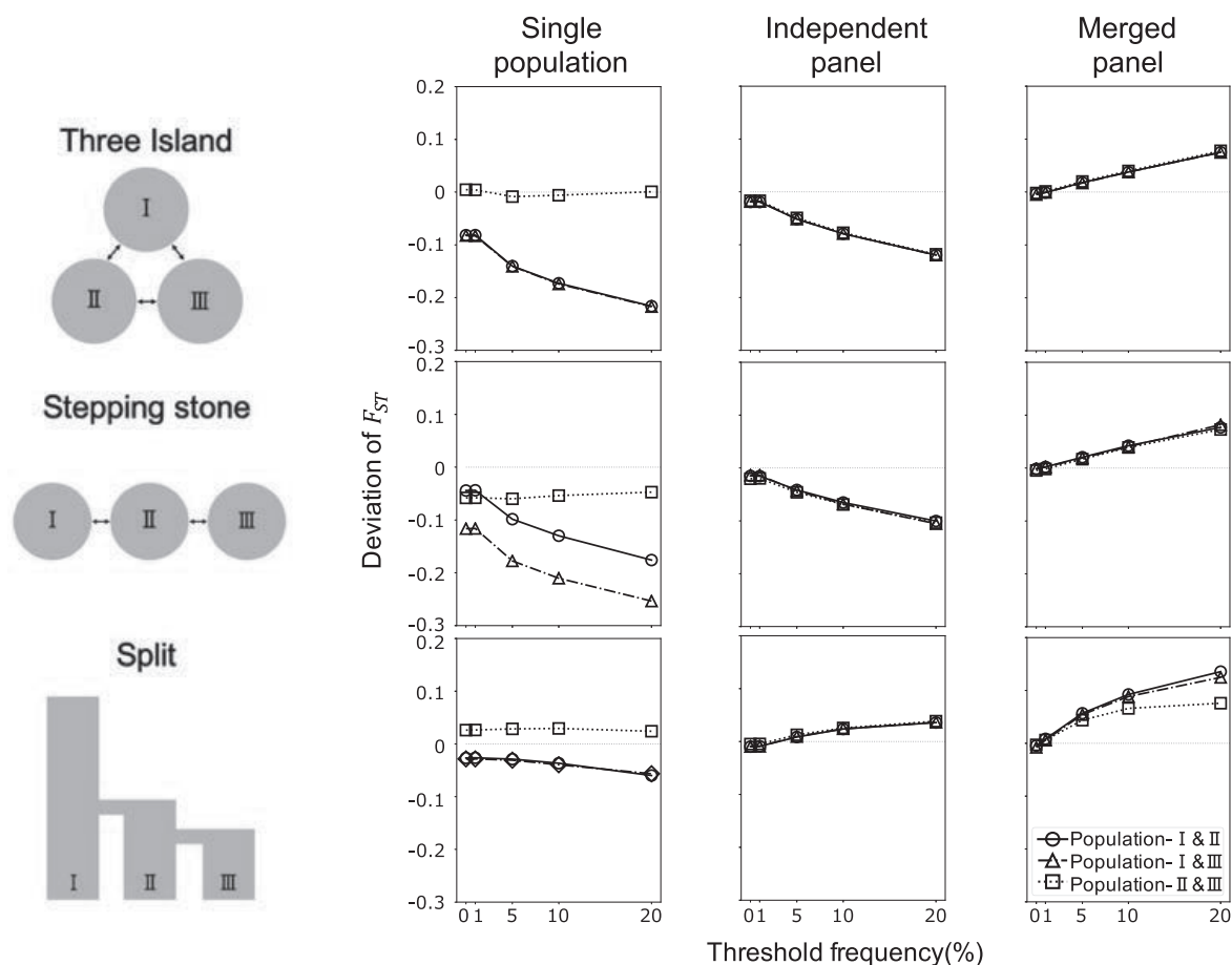
Figure 4 \hat{F}_{ST} under the combined effect of ascertainment schemes and population demography. The combined effect of ascertainment schemes and population demography on \hat{F}_{ST} estimation. Deviations of \hat{F}_{ST} from the estimates with re-sequencing data are plotted against the threshold of marker selection in each ascertainment scheme. \hat{F}_{ST} deviations between population-I and -II, -I and -III, and -II and -III are indicated by circles, triangles, and squares, respectively. The average \hat{F}_{ST} values calculated from the re-sequencing data for each demographic model are summarized in Supplementary Table S3.
