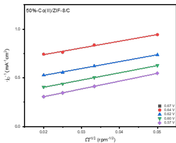
Fig. S2: Koutecky-Levich plots determined from Figure 1a-c of the modified ZIF-8 at different electrode potential values
