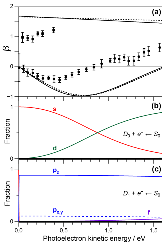
FIG. 2. (a) Photoelectron anisotropy parameters, \beta , evaluated from the photoelectron images for the D_0(^2\Sigma_u^+) + e^- \leftarrow S_0(^1\Sigma_g^+) (circles) and D_1(^2\Sigma_g^+) + e^- \leftarrow S_0(^1\Sigma_g^+) transitions (squares) of \text{Ag}_3^- as a function of photoelectron kinetic energy. The results of the simulation are superimposed by the solid and dashed curves, which are obtained by ezDyson 5.0 using EOM-IP-CCSD/aug-cc-pVDZ-PP and BP86/LanL2DZ levels of calculation, respectively (see the text). (b) and (c) Partial wave analyses for photoelectrons ejected via the D_0(^2\Sigma_u^+) + e^- \leftarrow S_0(^1\Sigma_g^+) and the D_1(^2\Sigma_g^+) + e^- \leftarrow S_0(^1\Sigma_g^+) transitions, respectively, obtained by the EOM-IP-CCSD/aug-cc-pVDZ-PP level of calculation.
