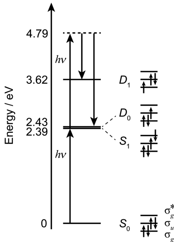
FIG. 5. Energy diagram of the two-photon detachment via the S_1(^1\Sigma_u^+) state of \text{Ag}_3^- .
