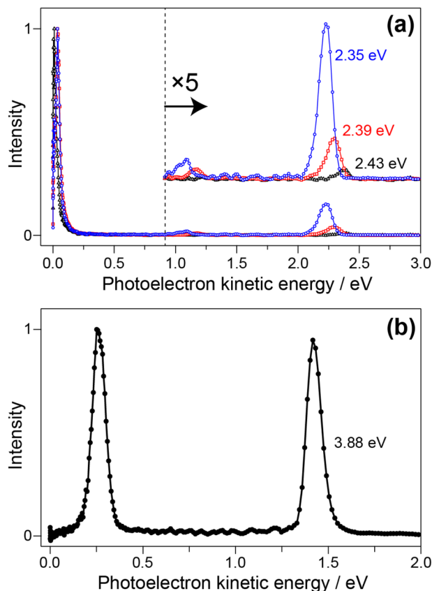
FIG. 6. (a) Photoelectron spectra of \text{Ag}_3^- obtained by the detachment laser at 2.35 (blue circles), 2.39 (red squares), and 2.43 eV (black triangles). (b) Photoelectron spectrum of \text{Ag}_3^- obtained at 3.88 eV. The intensity is in arbitrary units.
