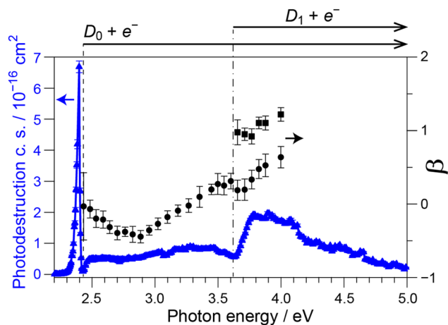
FIG. 4. Photodestruction action spectrum (blue triangles) of \text{Ag}_3^- obtained at an ion trap temperature of 100 K, 10 along with the \beta values for the D_0(^2\Sigma_u^+) + e^- \leftarrow S_0(^1\Sigma_g^+) (circles) and D_1(^2\Sigma_g^+) + e^- \leftarrow S_0(^1\Sigma_g^+) transitions (squares) plotted as a function of photon energy. The vertical dashed line shows the VDE, while the dash-dotted line indicates the second detachment threshold.
