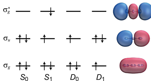
FIG. 3. Leading electronic configurations of S_0 , S_1 , D_0 , and D_1 states for anionic and neutral silver trimers along with the iso-surface plots of \sigma_g , \sigma_u , and \sigma_g^* MOs formed mainly with 5s atomic orbitals of silver atoms. The plots were obtained by the BP86/LanL2DZ level of calculation.
