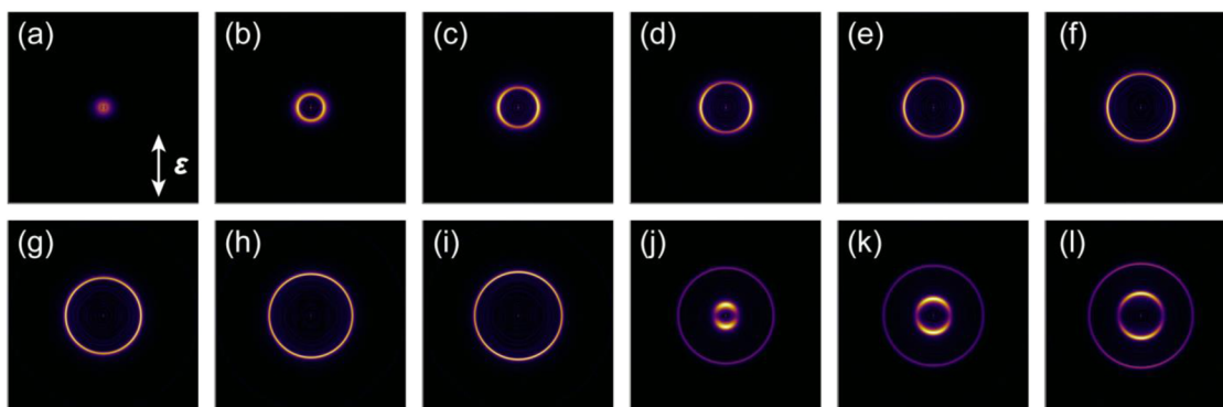
FIG. 1. 2D slices of photoelectron distributions for \text{Ag}_3^- obtained at (a) 2.43, (b) 2.53, (c) 2.64, (d) 2.76, (e) 2.89, (f) 3.02, (g) 3.18, (h) 3.35, (i) 3.45, (j) 3.65, (k) 3.77, and (l) 3.88 eV. The direction of the polarization vector, \epsilon , of the photodetachment laser is indicated by a double arrow in (a). The original projected images before transformation to these 2D slices can be found in Fig. S3 in the supplementary material .
