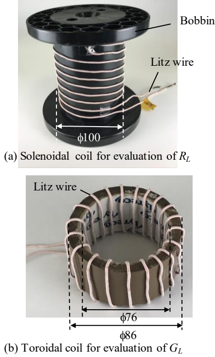
Fig. 5. Photographs of the experimental setup for evaluation of the loss coefficient R_L and G_L .
