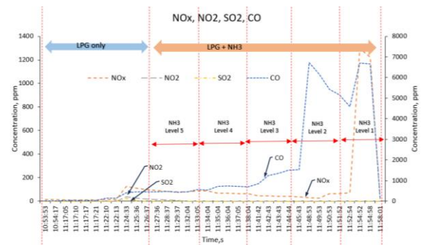
Fig. 5: Emission gas concentration at the discharge of combustion chamber during LPG and co-firing Ammonia
