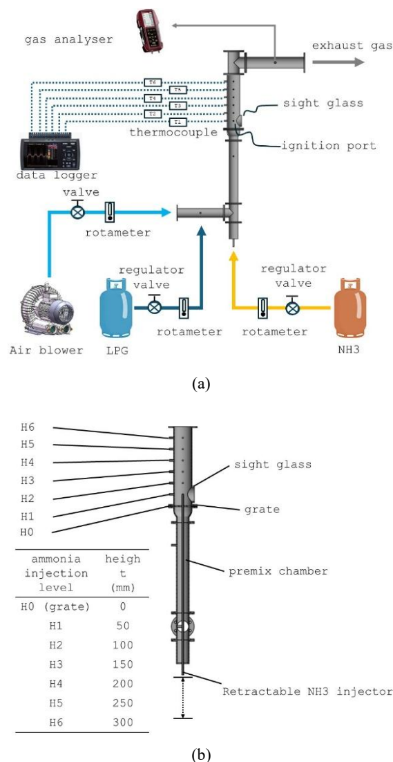
Fig. 3: (a) Experimental set-up (b) Combustion chamber and \text{NH}_3 injection system
