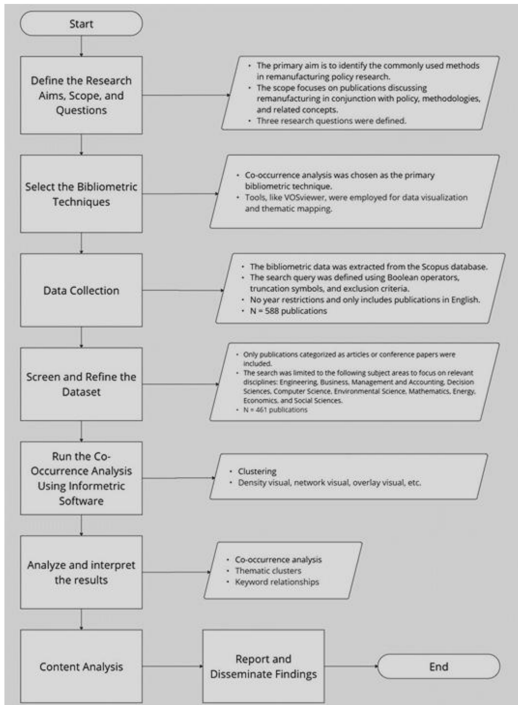
Fig. 3: Research Methodology
