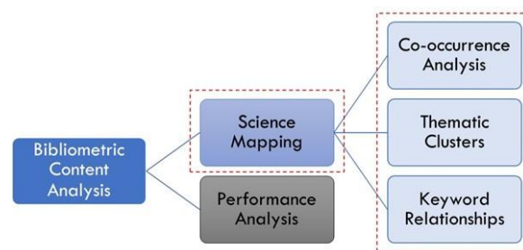
Fig. 2: Conceptual Framework
