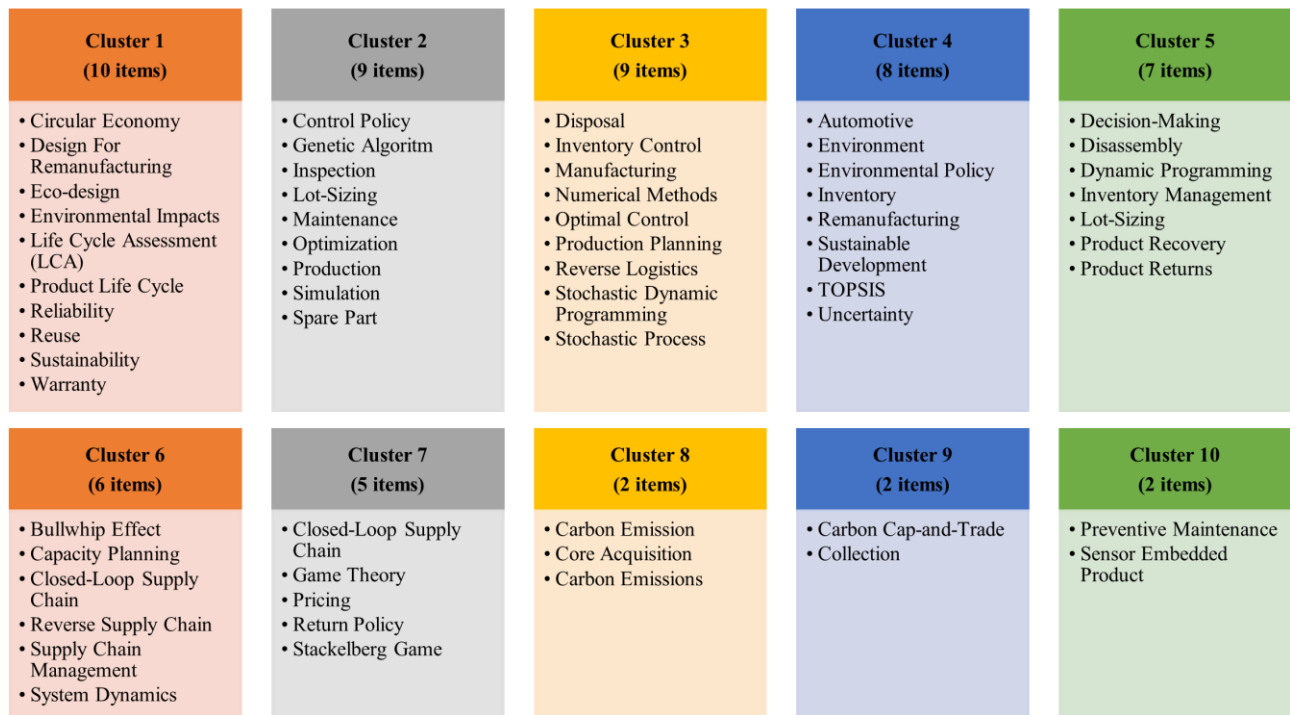
Fig. 4: Thematic Clustering
