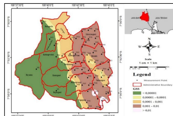
Fig. 5: Map of Ground shear strain ( \gamma ) in Padaherang Subdistrict
