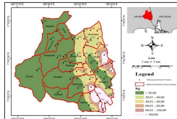
Fig. 4: Map of Seismic vulnerability (Kg) in Padaherang Subdistrict
