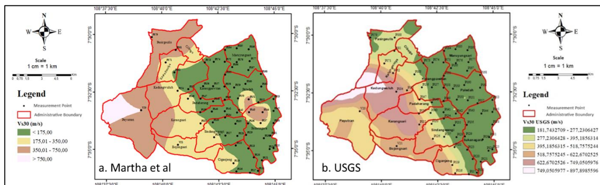
Fig. 6: (a) The map of Shear wave velocity ( V_s ) values at a depth of 30 meters from the inversion processing and (b) V_{S30} Distribution Map by USGS in Padaherang Subdistrict
