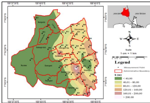
Fig. 7: Map of thickness of sediment layers (h) in Padaherang Subdistrict
