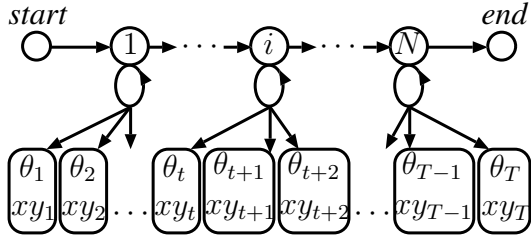
Figure 3. xy\theta -HMM.
