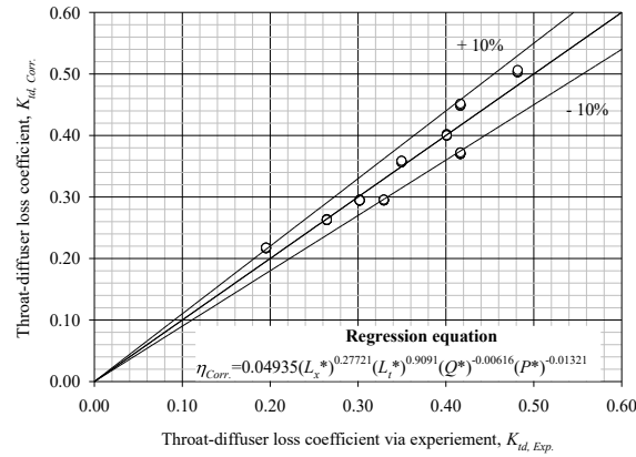
Fig. 5: Comparison of regression equations for throat diffuser loss coefficient with present experimental data
