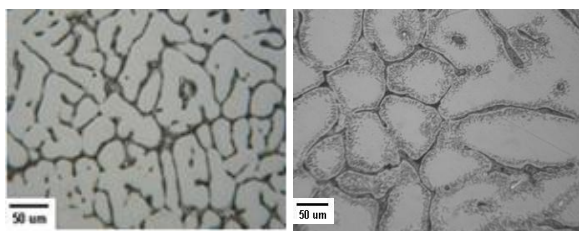
(a) (b) Fig. 2: Optical microscope images of the Al-5%Cu-4%Mg matrix without SiC reinforcement: (a) as-cast microstructure showing a dendritic grain morphology, and (b) microstructure after semi-solid processing, showing the transformation into a globular grain structure
