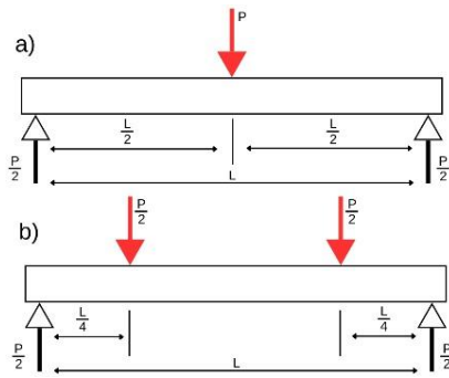
Fig. 5: Scheme of bending test (a) three-point bending, and (b) four-point bending
