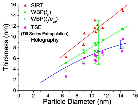
FIG. 7. (Color online) The relation between particle diameter and thickness (height) for the FePd nanoparticles estimated by using several different techniques. The large error bar for WBP indicates a possible elongation of d_z = 4.1 nm, as suggested by Eqs. (2) and (3).
