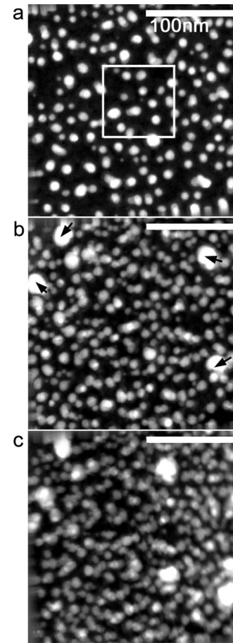
FIG. 1. Z-contrast images acquired during a tilt-series observation, after tilt-axis correction. (a) \alpha=0^\circ , (b) \alpha=-66^\circ , and (c) \alpha=+64^\circ . The tilt series was observed sequentially from 0^\circ to -70^\circ and then 0^\circ to +70^\circ . The reconstructed area, 75 \times 75 \text{ nm}^2 in size, is also indicated in Fig. 1(a). Large Cu particles are indicated by arrows in Fig. 1(b).
