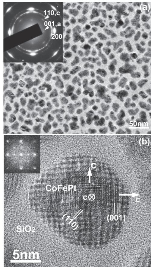
Fig. 5. (a) BF-TEM image and the corresponding SAED pattern of the (\text{Co}_{26}\text{Fe}_{20})\text{Pt}_{44}\text{-Ag}_{10}\text{-SiO}_2 nanocomposite thin film formed at 675 K with a sputtering power of 90 W. (b) HRTEM image and the corresponding FFT pattern of a nanoparticle with a three-variant ordered domain structure.
