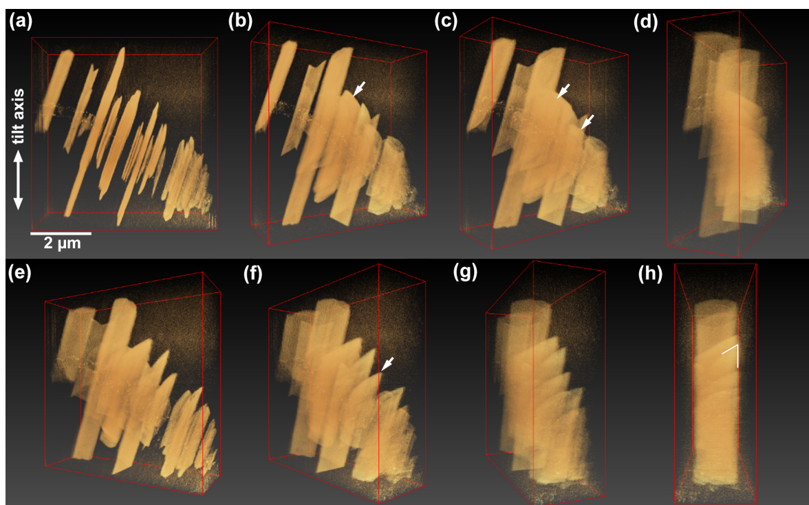
Fig. 3 Reconstructed 3D volumes of a \text{Mg}_{97}\text{Zn}_1\text{Gd}_2 cast alloy after aging at 773 K for 18 ks. The reconstructed volume is 5665 \text{ nm} \times 5857 \text{ nm} \times 1989 \text{ nm} with the pixel size of 5.8 nm/pixel. The foil thickness is \sim 1700 \text{ nm} . Tilt angle with respect to the original tilt axis is as follows: (a) 0^\circ , (b) 30^\circ , (c) 50^\circ , (d) 70^\circ , (e) -30^\circ , (f) -50^\circ , (g) -70^\circ , (h) -90^\circ .
