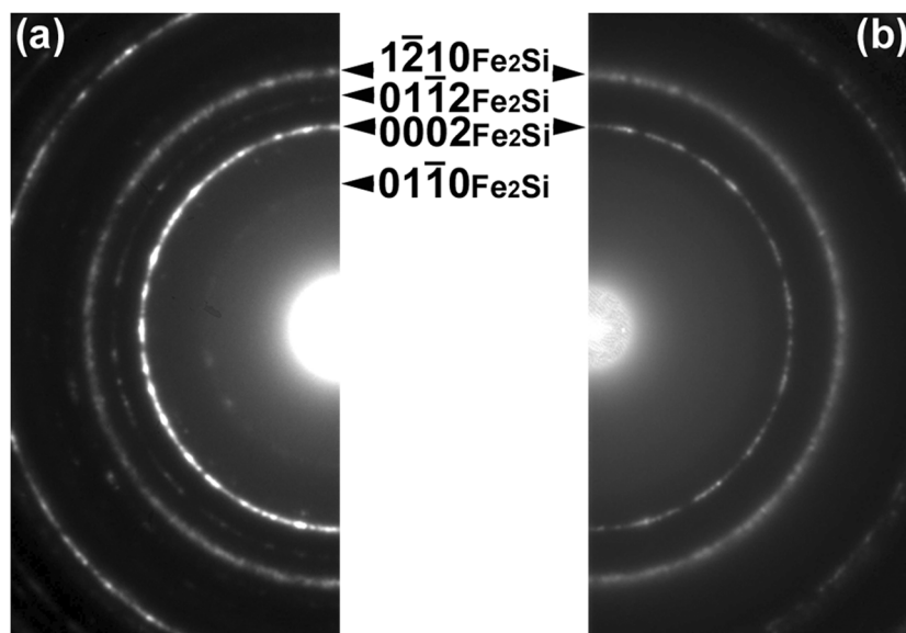
Fig. 12. SAED patterns obtained for a-SiO x /Fe/a-SiO x (a) and a-SiO 2 /Fe/a-SiO 2 (b) thin films after 75 keV electron irradiation at 298 K (total dose: 1.0 \times 10^{28} e/m 2 ). Reprinted from Supporting Information of Sato and Fujii [22].
