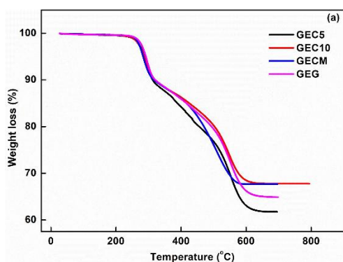
Fig. 8: TGA thermograms: (a) weight loss and (b) derivative weight of the composites
