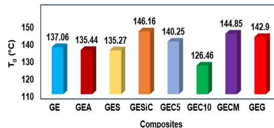
Fig. 6: The T_g of hybrid composites
