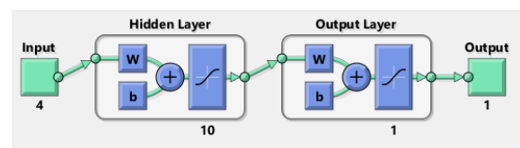
Fig. 2: ANN Network Architecture
