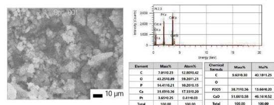
Fig. 3a: SEM-EDS of HA microparticle
