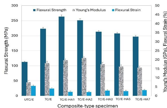
Fig. 7: Flexural strength, flexural modulus, and flexural strain of C/E-HA composite-type specimens
