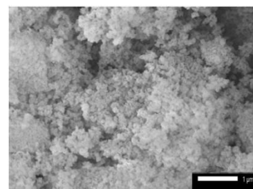
Fig. 3b: SEM micrograph of HA microparticle, showing a clustering trend of particles
