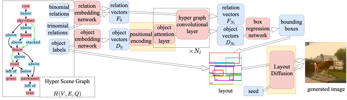
Figure 5: Example of generating an image with OA-hsg2im. The modified parts from hsg2im (Miyake et al., ) are highlighted in yellow. N_l (= 12) is the number of object attention layers and graph convolutional layers.
