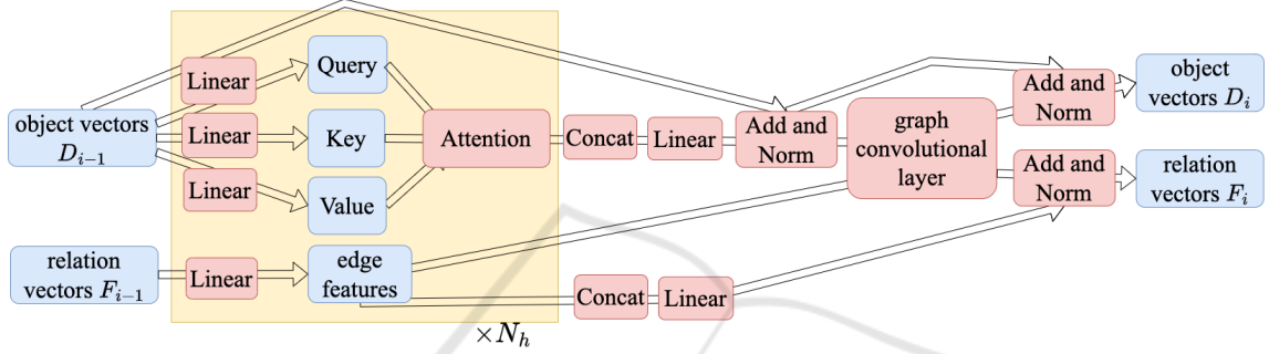
Figure 6: Flow of the i -th object attention layer and hyper graph convolutional layer. In the Add and Norm, we perform the batch normalization to the add-sum of the two input vectors. In the Concat, we concatenate the object vectors obtained from each head of attention.
