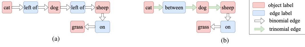
Figure 2: Example of a scene graph (a) and a hyper scene graph (b). This Figure is from (Miyake et al., ). Set V of objects are the same in both (a) and (b), and they are given by V = \{\text{cat}, \text{dog}, \text{sheep}, \text{grass}\} . The set of the binomial edges in (a) and (b) are given by E = \{(v_1, r_1(\text{left of}), v_2), (v_2, r_2(\text{left of}), v_3), (v_3, r_3(\text{on}), v_4)\} and E = \{(v_3, r_3(\text{on}), v_4)\} , respectively. The set of the trinomial hyperedges in (b) is given by Q = \{(v_1, r_4(\text{between}), v_2, v_3)\} . The path \text{cat} \rightarrow \text{left of} \rightarrow \text{dog} corresponds to the binomial edge (v_1(\text{cat}), \text{left of}, v_2(\text{dog})) and represents that a cat is located to the left of a dog. Also, the path \text{cat} \rightarrow \text{between} \rightarrow \text{dog} \rightarrow \text{sheep} corresponds to the trinomial edge (v_1(\text{cat}), \text{between}, v_2(\text{dog}), v_3(\text{sheep})) and represents from left to right, a cat, a dog, and a sheep aligned in a row.
