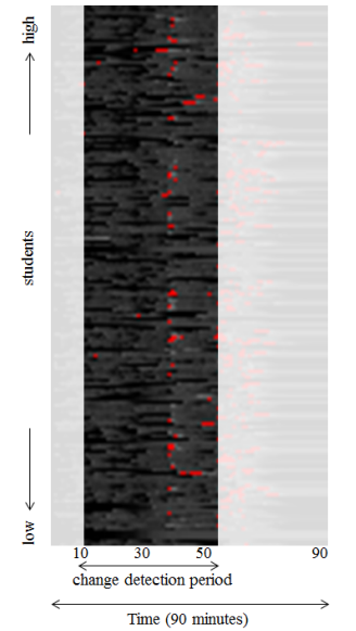
Figure 3: Anormal score of students over time, with brighter colors reflecting larger value of A_{i,t} . The red color indicates the change detection results.
