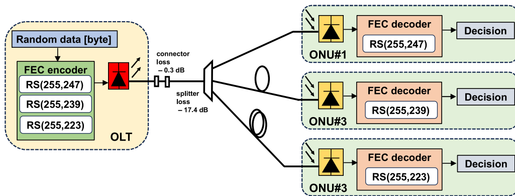
Fig. 2 The transmission model of the PON under investigation
