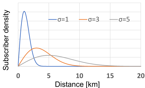
Fig. 3 Subscriber density distribution
