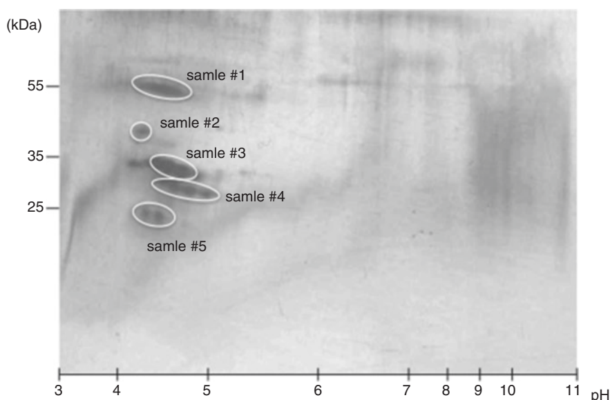
Fig. 5.2 2D-PAGE profile of P. flavoviridis venomous fang matrix proteins Samples #1 to #5 were analyzed by nanoLC-MALDI-TOF MS/MS analysis after in-gel digestion, respectively
