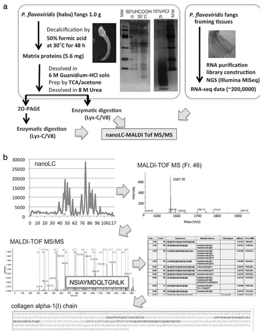
Fig. 5.1 Proteomic analysis of P. flavoviridis fang matrix proteins Brief explanation of procedure through decalcification and mass spectrometry analysis (a) and typical profiles of digested matrix proteins on nanoLC-MALDI-TOF MS/MS (b)
