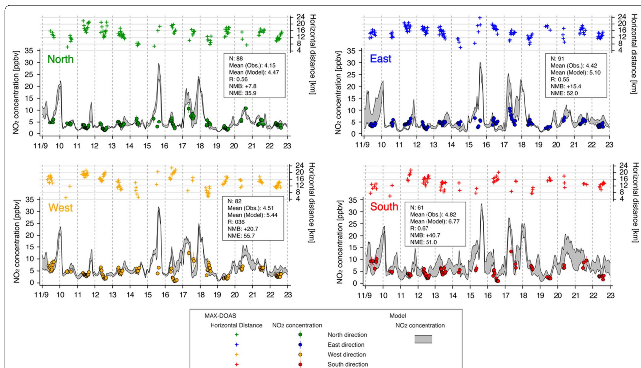
Fig. 5 Temporal variation of \text{NO}_2 concentration by MAX-DOAS and model averaged over 0–1 km (each direction). The MAX-DOAS measured horizontal distance is also plotted. The range of model results showed simulated \text{NO}_2 concentration within 4–24 km from Chiba University in each direction. Statistical scores are shown in the inset, and 1 h averaged MAX-DOAS observation and corresponded horizontal distance to observation were used for this analysis
