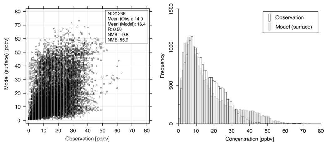
Fig. 3 (Left) Scatter-plot of hourly surface level \text{NO}_2 concentration during Chiba-Campaign 2015. (Right) Histogram for observations (white) and the model (gray). Ground-based observation by AEROS and the model are shown. AEROS sites located within 24 km of Chiba University (see, Fig. 1) are used
