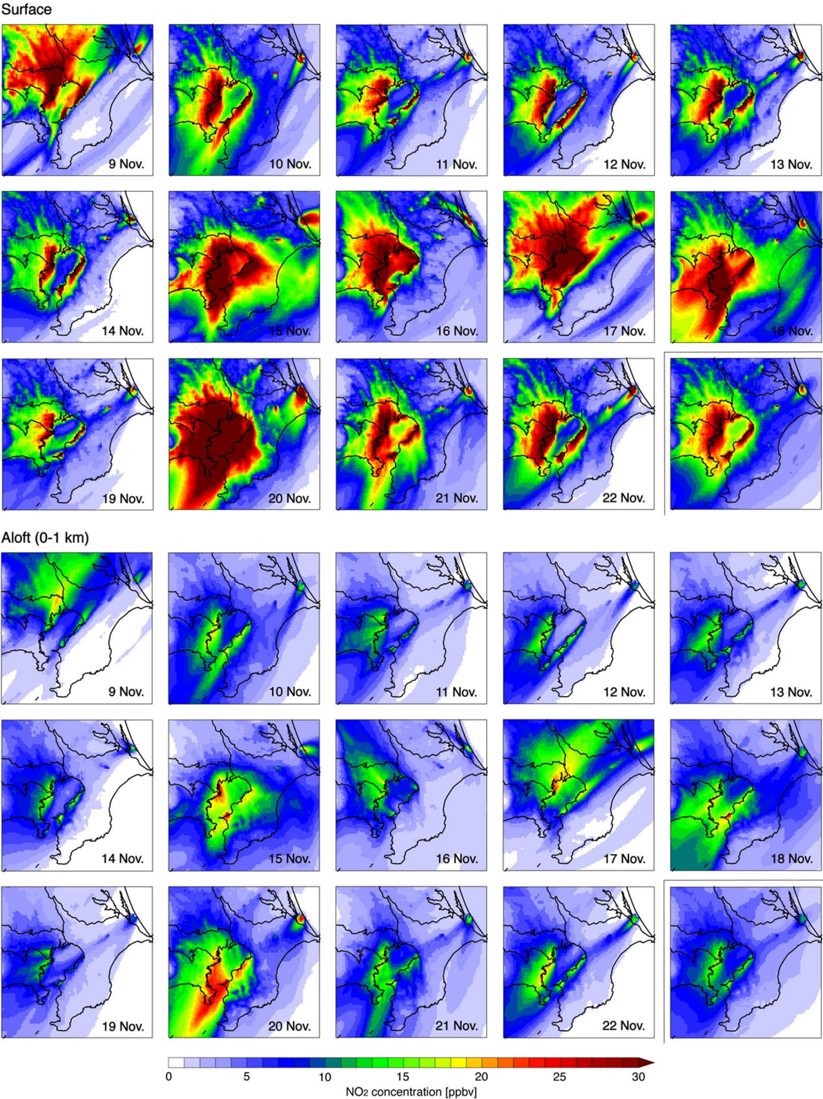
Fig. 9 Spatial distribution of modeled daily NO 2 concentration at surface and aloft (averaged over 0–1 km). The right-bottom panel shows the period average over the Chiba-Campaign 2015
