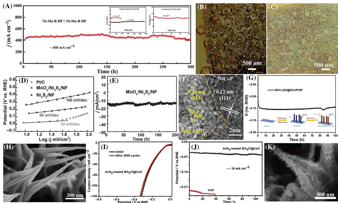
FIGURE 15 (A) The overall water splitting stability test of Ni-Mo-B HF at 450 \text{ mA cm}^{-2} in 1 M KOH. Insets are the stability test at 1, 2, and 5 \text{ A cm}^{-2} . Optical photos of \text{H}_2 bubbles attached to catalysts at low current density ( 20 \text{ mA cm}^{-2} ). (B) Pure nickel foam. (C) Ni-Mo-B HF. Reproduced with permission. 195 Copyright 2021, Wiley-VCH. Electrochemical testing of \text{MoO}_x/\text{Ni}_3\text{S}_2/\text{NF} . (D) Tafel plots. (E) I-t curve at an overpotential of 110 mV in 1 M KOH. Reproduced with permission. 196 Copyright 2016, Wiley-VCH. (F) HRTEM image of the NiFe LDH@NiCoP nanowire highlighting the interface between nanowire and nanosheets. (G) Long-term stability of the NiFe LDH@NiCoP/NF at 10 \text{ mA cm}^{-2} . Inset is the synthesis route of electrodes. Reproduced with permission. 202 Copyright 2018, Wiley-VCH. Physical characterization and electrochemical testing of Ar/ \text{H}_2 -treated \text{WO}_3/\text{C}@\text{CoO} . (H) SEM image. (I) The LSV curves before and after 2000 cycles. (J) The chronopotentiometry curve at 10 \text{ mA cm}^{-2} . (K) SEM image after the HER stability test. Reproduced with permission. 200 Copyright 2018, Elsevier
