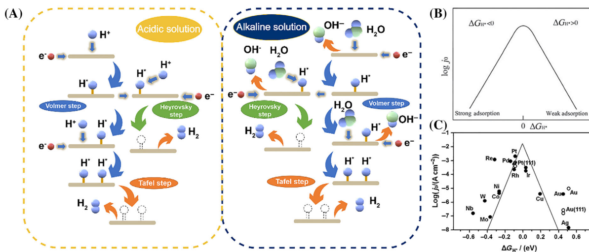
FIGURE 2 (A) Chemical processes in HER under acidic and alkaline conditions. (B) Relationship between the exchange current density ( j_0 ) and hydrogen adsorption free energy under the assumption of the Langmuir adsorption model. Reproduced with permission. 52 Copyright 1958, Royal Society of Chemistry. (C) Volcano plot of the relationship between the exchange current density ( j_0 ) and the free energy of hydrogen adsorption ( \Delta G_{H^*} ) for the surfaces of various metals. Reproduced with permission. 53 Copyright 2005, IOP Publishing
