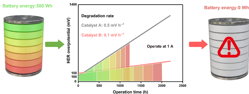
FIGURE 3 Proposed schematic stability test of Catalyst A (overpotential of 100 mV and degradation rate of 0.5 \text{ mV h}^{-1} ) and Catalyst B (overpotential of 150 mV and degradation rate of 0.1 \text{ mV h}^{-1} ) at a current of 1 A. Battery energy of 500 Wh allows Catalyst B to operate continuously for 2000 h but only allows Catalyst A to operate for 1228 h
