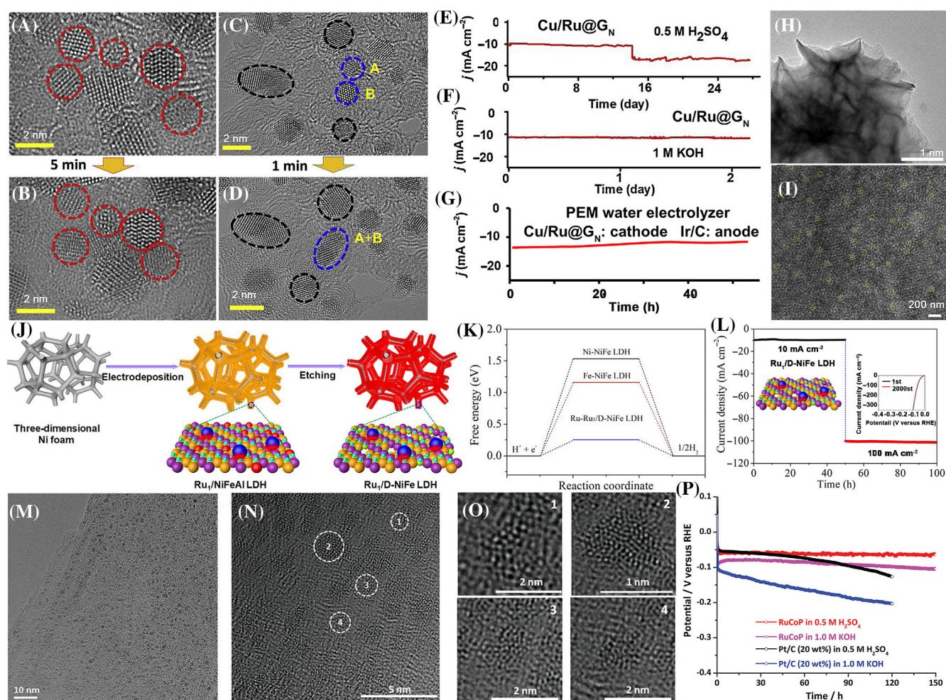
FIGURE 6 Continuous HRTEM analysis. (A–B) for \text{Cu/Ru}@G_N , (C–D) for \text{Ru}@G_N . Long-term stability test of \text{Cu/Ru}@G_N . (E) 0.5 \text{ M H}_2\text{SO}_4 . (F) 1 \text{ M KOH} . (G) PEM water electrolyzer. Reproduced with permission. 90 Copyright 2020, Elsevier. Synthetic schematic and morphological characterization of \text{Ru}_1/\text{D-NiFe LDH} . (H) TEM image. (I) Aberration-corrected TEM image. (J) Synthesis illustration. (K) Free energy diagram of HER process on different active sites. (L) Time-dependent current density curves at -0.018 and -0.061 \text{ V} versus RHE. Inset is LSV curves before and after 2000 cycles. Reproduced with permission. 93 Copyright 2021, Springer Nature. Structural morphology and stability analysis of \text{RuCoP} . (M) TEM. (N) HRTEM. (O) HRTEM images of individual clusters denoted in (N). (P) At 10 \text{ mA cm}^{-2} in 0.5 \text{ M H}_2\text{SO}_4 and 1 \text{ M KOH} , respectively. Reproduced with permission. 92 Copyright 2018, The Royal Society of Chemistry
