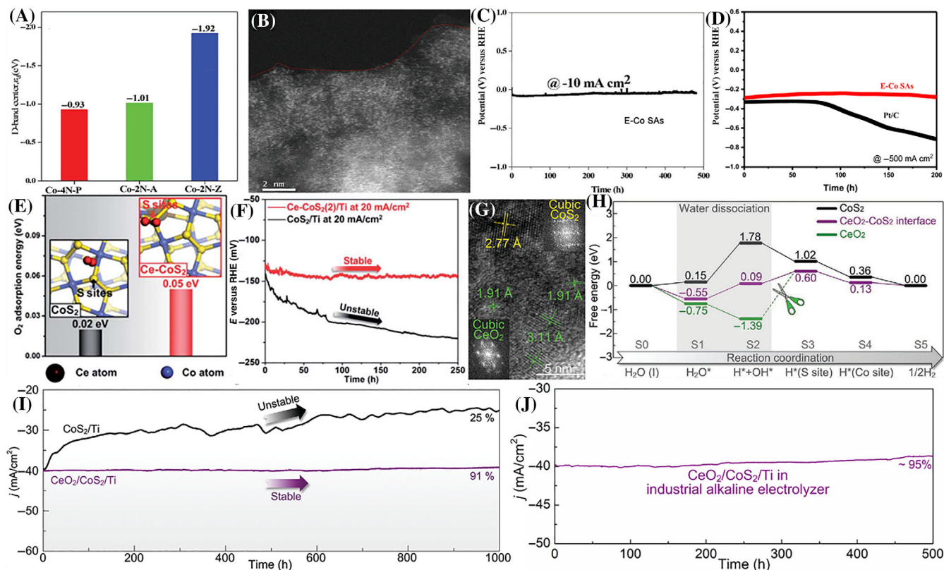
FIGURE 11 (A) The d-band center of Co-4N-P, Co-2N-A, and Co-2N-Z systems. (B) HAADF-STEM image of the E-Co SAs. (C) Time-dependent overpotential curve of E-Co SAs obtained at 10 \text{ mA cm}^{-2} in 1 M KOH. (D) Stability test at 500 \text{ mA cm}^{-2} for 200 h. Reproduced with permission. 164 Copyright 2021, Wiley-VCH. (E) \text{O}_2 adsorption energy on the S sites adjacent to Ce for Ce-CoS 2 . (F) Time-overpotential profiles at 20 \text{ mA cm}^{-2} in 1 M KOH. Reproduced with permission. 165 Copyright 2019, The Royal Society of Chemistry. Physical characterization and electrochemical test of CeO 2 /CoS 2 /Ti. (G) High-resolution TEM image. (H) Calculated free energy diagram for HER. (I) Catalytic durability at 40 \text{ mA cm}^{-2} in 1 M KOH. (J) Catalytic durability through a time-overpotential profile in 1 M KOH at 60^\circ\text{C} . Reproduced with permission. 163 Copyright 2021, Wiley-VCH
