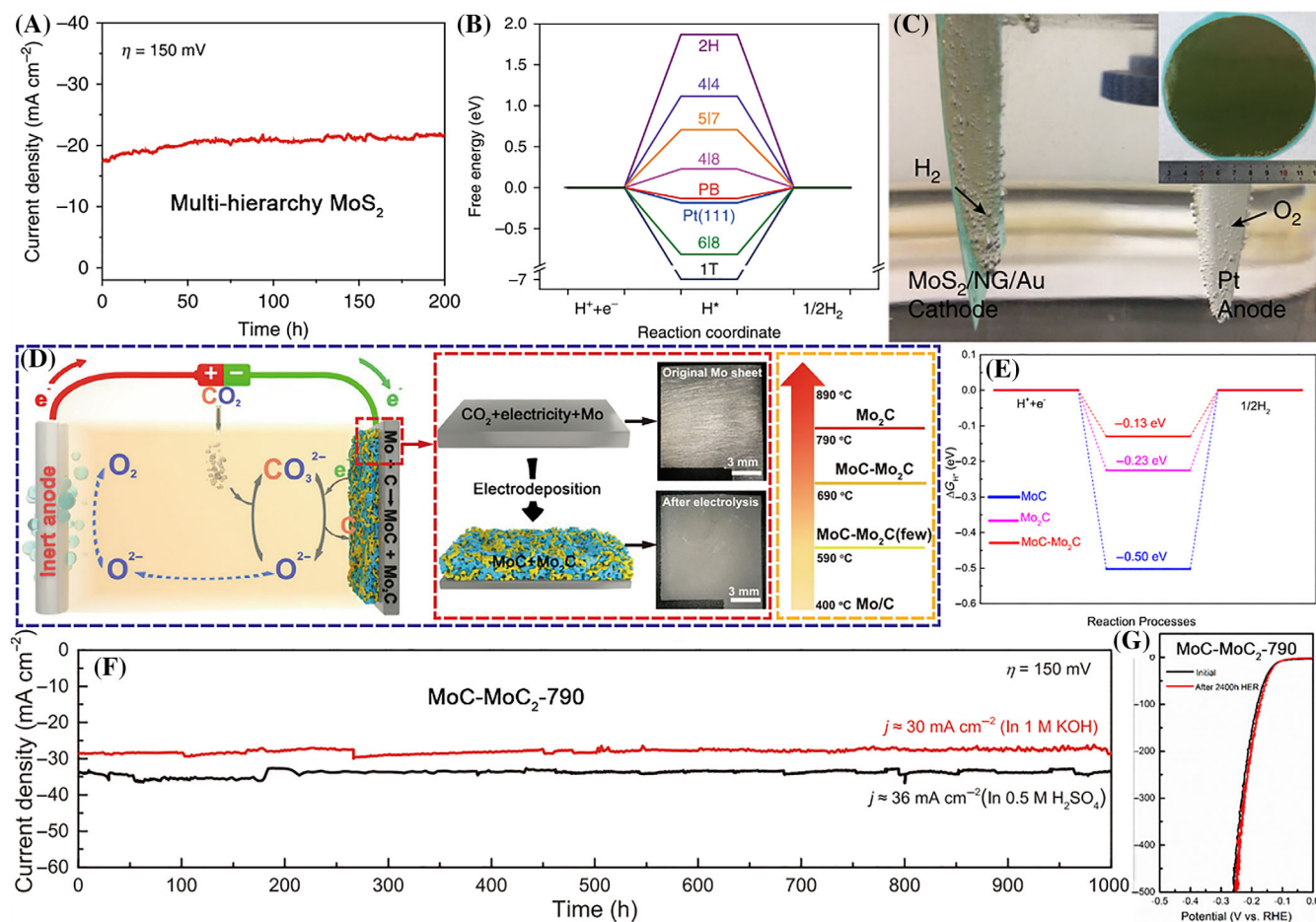
FIGURE 13 (A) I-t curve of a multi-hierarchy \text{MoS}_2 catalyst under the overpotential of 150 mV in 0.5 M \text{H}_2\text{SO}_4 . (B) A comparison of the Gibbs free energies of the adsorbed H on 2H–1T-phase boundaries (PBs) and other samples. (C) Digital photograph of HER of multi-hierarchy \text{MoS}_2 catalyst under acidic electrolyte. Inset: Picture of multi-hierarchy \text{MoS}_2 catalyst with a diameter of 4 inches. Reproduced with permission. 182 Copyright 2019, Springer Nature. (D) Schematic diagram of \text{MoC-Mo}_2\text{C-790} prepared by molten carbonate and digital photos of Mo electrodes before and after electrolysis. (E) Calculated \Delta G_{\text{H}^*} diagram of the HER in acid electrolyte. (F) The long-term electrolysis stability test of \text{MoC-Mo}_2\text{C-790} at \eta = 150 mV in 0.5 M \text{H}_2\text{SO}_4 and 1 M KOH. (G) LSV polarization curves before and after 2400 h stability test. Reproduced with permission. 181 Copyright 2021, Springer Nature
