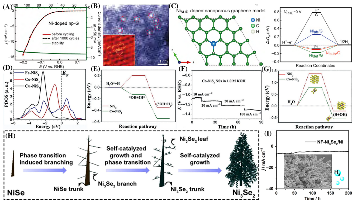
FIGURE 9 (A) Stability of Ni-doped np-G at the overpotential of 150 mV in 0.5 M \text{H}_2\text{SO}_4 . Inset is LSV curves before and after 1000 cycles. (B) HAADF-STEM image of Ni-doped np-G. (C) Hydrogen adsorption sites and configuration of the \text{Ni}_{\text{sub}}/\text{G} model with \Delta G_{\text{H}^*} = -0.10 eV (left) and calculated Gibbs free energy diagram (right). Reproduced with permission. 142 Copyright 2015, Wiley-VCH. (D) Partial density of states (PDOS) of 3d-bands of Co, Fe, and Cu dopants. (E) Energetic pathway of HER. (F) Chronoamperometric response of the Co-NiS 2 NSs at different current densities. (G) Transition state barrier for H 2 O-splitting; Insets are models for *H 2 O and *H + adsorbed on NiS 2 and Co-NiS 2 NSs. Reproduced with permission. 144 Copyright 2019, Wiley-VCH. (H) Schematic diagram of the preparation of Ni 3 Se 2 nanoforest on Ni foam. (I) Durability of NF-Ni 3 Se 2 /Ni at -0.200 V versus RHE in 1 M KOH. Inset is the SEM image after the HER stability test. Reproduced with permission. 49 Copyright 2016, Elsevier
