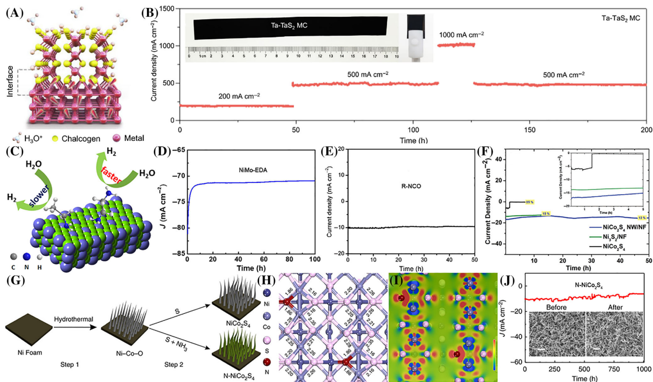
FIGURE 14 (A) Atomic structure of the Ta-TaS 2 MC. (B) I - t curves of the Ta-TaS 2 MC at 200, 500, and 1000 mA cm -2 in a 0.5 M H 2 SO 4 electrolyte. Inset is a photograph of self-supporting electrode Ta-TaS 2 , about 35 cm 2 . Reproduced with permission. 44 Copyright 2021, Springer Nature. (C) Surface modification scheme of NiMo nanoparticles with EDA. (D) The durability test of NiMo-EDA under the overpotential of 300 mV in 1 M KOH. Reproduced with permission. 201 Copyright 2017, American Chemical Society. (E) The stability test of R-NCO with a constant voltage of 0.135 V in 1 M KOH. Reproduced with permission. 220 Copyright 2018, American Chemical Society. (F) Time-dependent current density curves of NiCo 2 S 4 NW/NF at a static potential of -0.323 V versus RHE for 50 h, in 1 M KOH. Reproduced with permission. 221 Copyright 2016, Wiley-VCH. (G) Schematic diagram of the preparation of N-NiCo 2 S 4 . (H) The top-view structures of N-NiCo 2 S 4 (100). (I) The top-view electron density difference of N-NiCo 2 S 4 (100), ranging from -0.1 to 0.1. (J) I - t curves of N-NiCo 2 S 4 recorded for 1000 h at 50 mV versus RHE in 1 M KOH. Inset is the SEM images for N-NiCo 2 S 4 before and after the stability test, and the scale bar is 1 μm. Reproduced with permission. 194 Copyright 2018, Springer Nature
