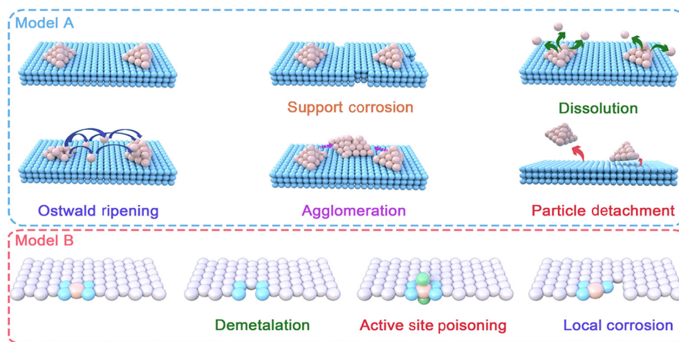
FIGURE 4 Degradation mechanisms of hydrogen evolution reaction (HER) catalysts
