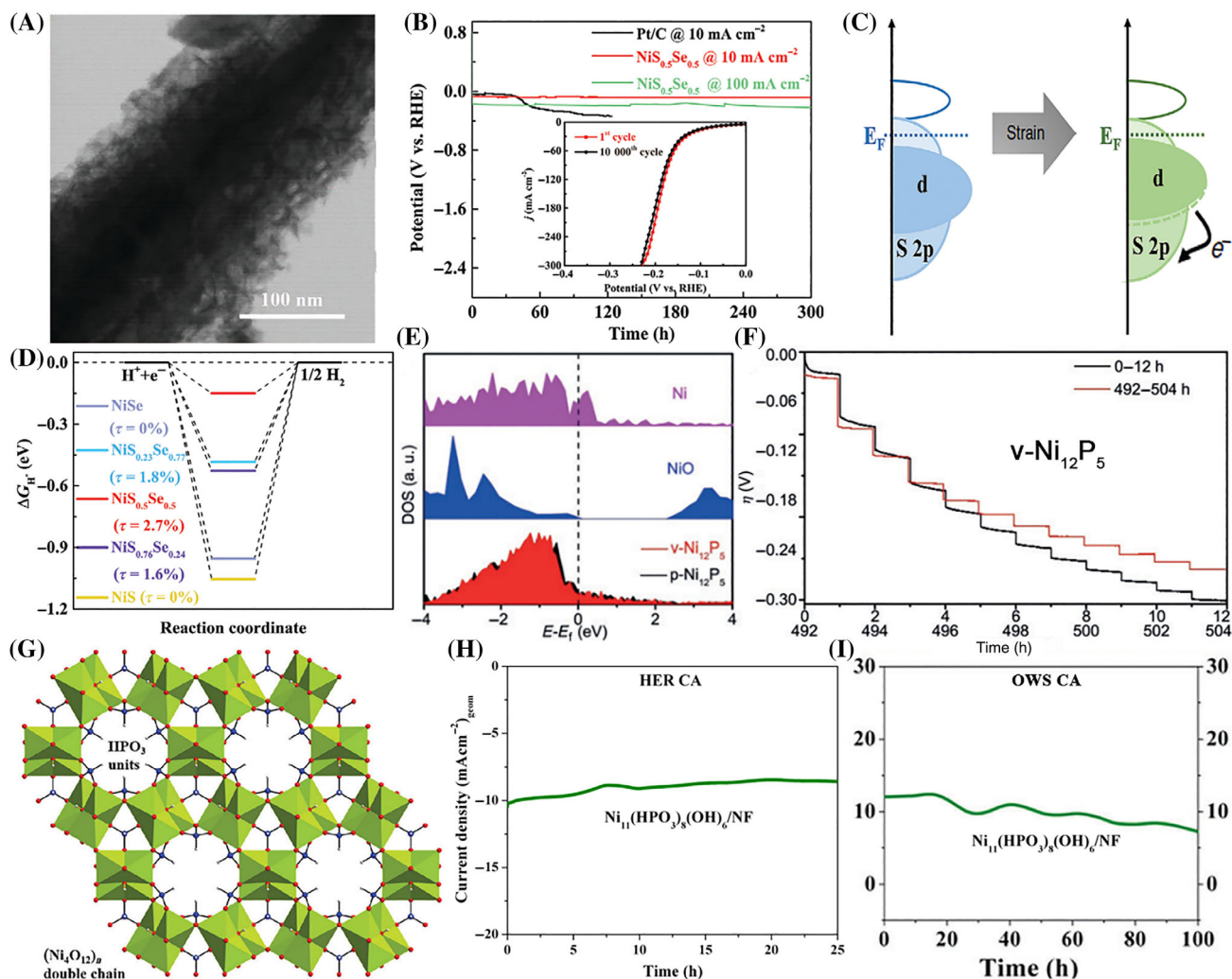
FIGURE 10 (A) TEM image of \text{NiS}_{0.5}\text{Se}_{0.5} . (B) Durability test of \text{NiS}_{0.5}\text{Se}_{0.5} at a current density of 10 and 100 \text{ mA cm}^{-2} in 1 \text{ M KOH} . Inset is LSV curves before and after 10 000 cycles. (C) Schematic of the electron exchange for the lattice-strained surface of \text{NiS}_{0.5}\text{Se}_{0.5} . (D) Gibbs free-energy diagram. Reproduced with permission. 140 Copyright 2020, Wiley-VCH. (E) The v\text{-Ni}_{12}\text{P}_5 and p\text{-Ni}_{12}\text{P}_5 catalysts of Ni 3d for density of states (DOS). (F) Chronoamperometry test of v\text{-Ni}_{12}\text{P}_5 in 1 \text{ M KOH} at various current densities ( 5, 10, 20, 30, 40, 50, 60, 70, 80, 90, 100 \text{ mA cm}^{-2} ). Reproduced with permission. 139 Copyright 2020, Wiley-VCH. (G) Crystal structure of \text{Ni}_{11}(\text{HPO}_3)_8(\text{OH})_6 . The long-term stability test of \text{Ni}_{11}(\text{HPO}_3)_8(\text{OH})_6/\text{NF} . (H) HER stability at an overpotential of 130 \text{ mV} in 1 \text{ M KOH} . (I) The overall water splitting stability at 1.65 \text{ V} versus RHE. Reproduced with permission. 143 Copyright 2018, The Royal Society of Chemistry
