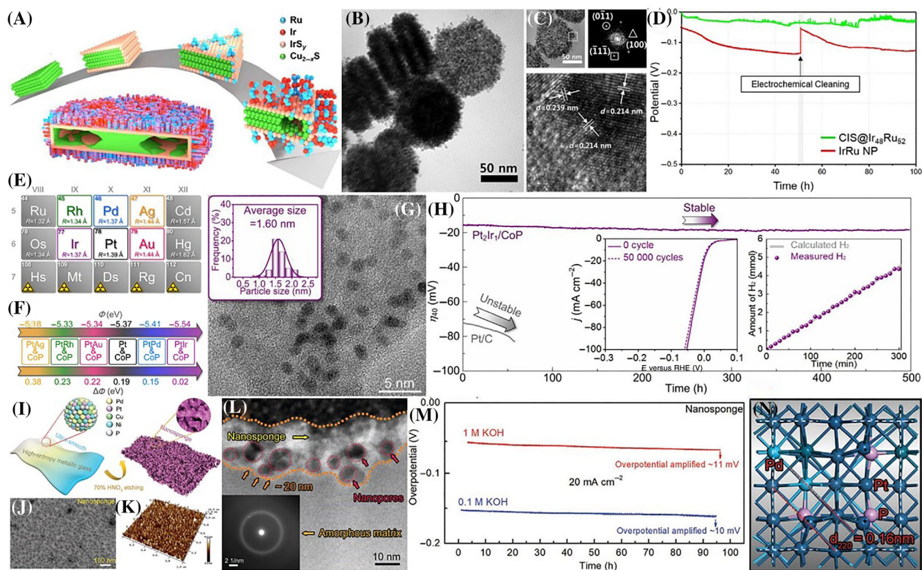
FIGURE 8 Synthetic route of CIS@Ir 48 Ru 52 and morphological characterization and stability test. (A) Schematic illustration. (B) TEM image. (C) HRTEM and magnified HRTEM image, corresponding to its FFT pattern with the zone axis of [011]. (D) HER stability in 0.1 M HClO 4 . Reproduced with permission. 127 Copyright 2018, The Royal Society of Chemistry. (E,F) The PtM/CoP catalysts with the controllable \Delta\phi . (G) TEM images for the Pt 2 Ir 1 /CoP. Inset is the size of the PtIr nanoparticle of \sim 1.60 nm on CoP nanosheets. (H) Long-term stability of Pt 2 Ir 1 /CoP through a time-overpotential profile at 40 mA cm -2 . Insets are cycle performance of LSV curves and Faradic efficiency. Reproduced with permission. 126 Copyright 2021, Springer Nature. Conceptional design and surface characterization of the nanoporous PdPtCuNiP HEMG. (I) Schematic illustration. (J) SEM image. (K) 3D AFM image. (L) Aberration-corrected HAADF-STEM image. Inset is the corresponding SAED pattern of the predominantly amorphous matrix. (M) The time-dependent HER stability at a current density of 20 mA cm -2 in 1 and 0.1 M KOH solutions. (N) DFT atomic modeling of the Pt 5 Pd 3 P 2 nanocrystals showing the lattice distortion caused by interstitial alloying of P. Reproduced with permission. 34 Copyright 2021, Wiley-VCH
