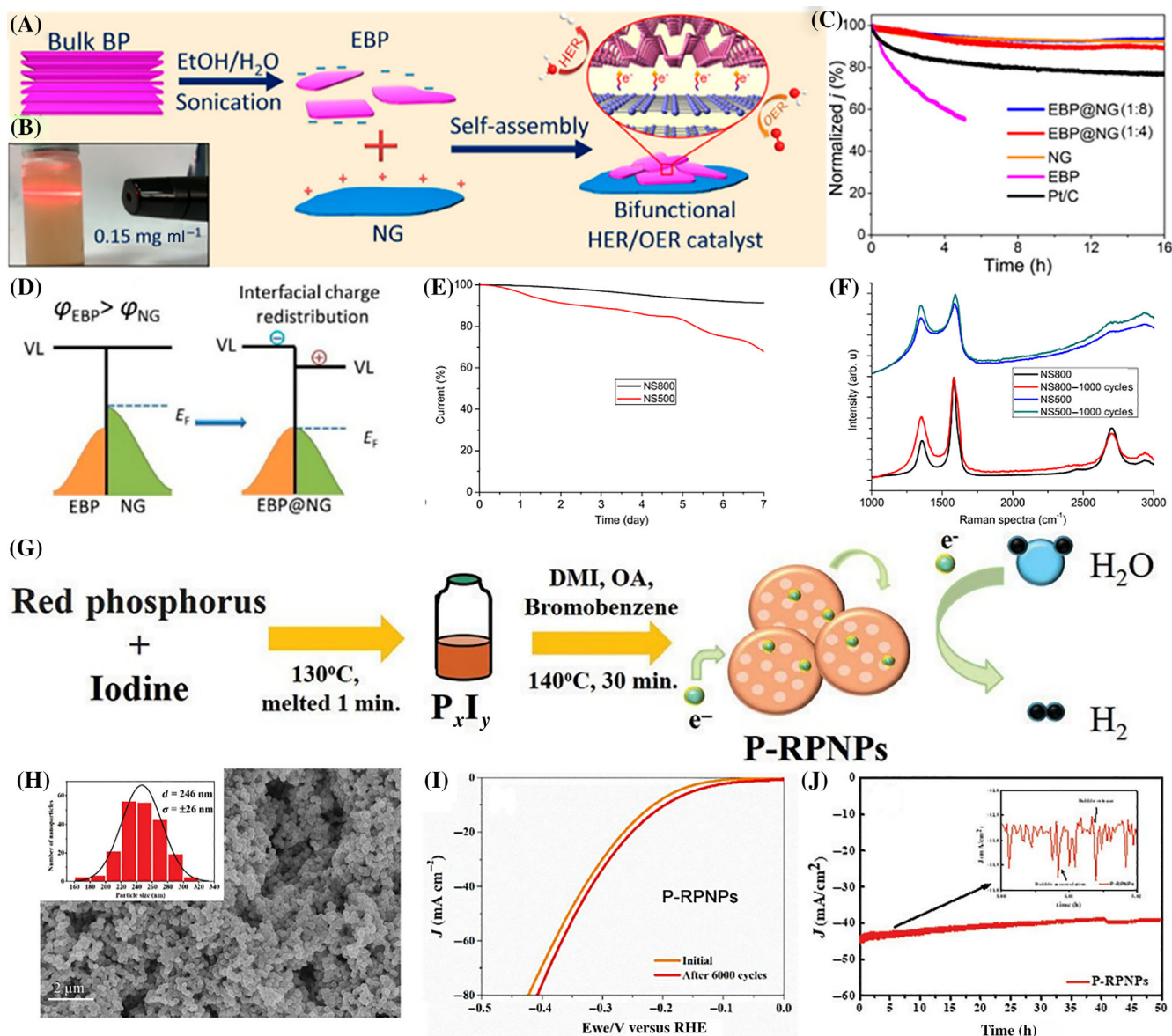
FIGURE 18 The EBP@NG catalyst: (A) Diagram of preparation process. (B) Photograph of an EBP dispersion with the concentration up to 0.15 mg ml -1 , showing a Tyndall effect. (C) Chronoamperometric curves of EBP@NG. (D) Illustration of interfacial charge redistribution between NG and EBP. Reproduced with permission. 36 Copyright 2019, American Chemical Society. NS-500 and NS-800: (E) HER activity. (F) Durability at -0.2 V. Reproduced with permission. 228 Copyright 2015, Wiley-VCH. P-RPNPs: (G) Diagram of preparation process. (H) SEM image, the inset shows the histograms of size distribution. (I) HER durability test at the voltage from 0.2 to -0.6 V for 6000 cycles in 0.5 M H 2 SO 4 . (J) Stability test at the current density of -0.5 V (vs. RHE) for 50 h. Reproduced with permission. 39 Copyright 2020, The Royal Society of Chemistry
