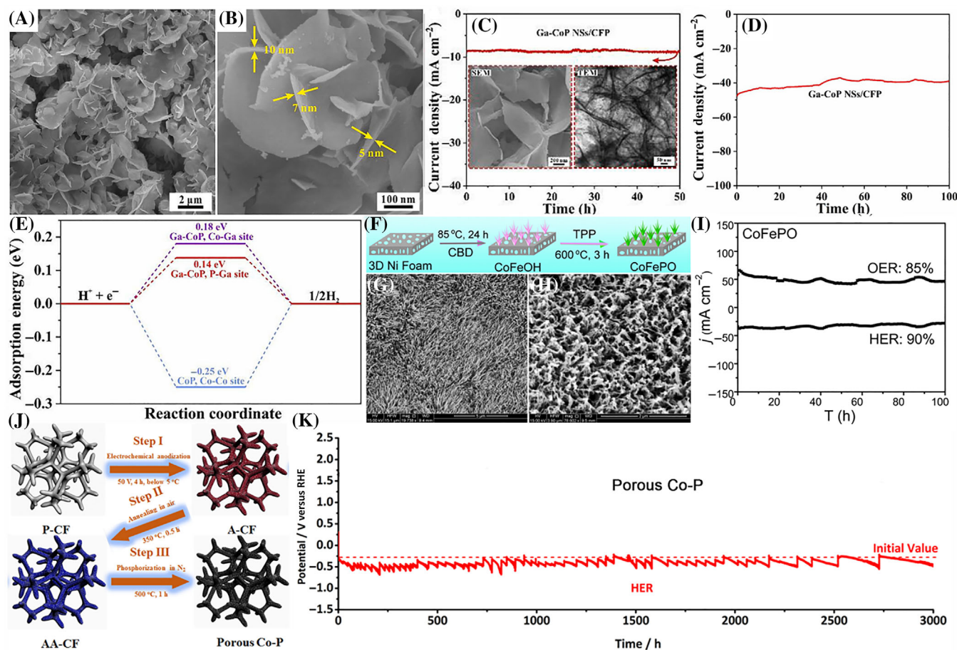
FIGURE 12 Morphological characterization and electrochemical stability testing of Ga-CoP NSs. (A) Low-magnification SEM. (B) High-magnification SEM. (C) I - t curve at 10 \text{ mA cm}^{-2} in 1 \text{ M KOH} . (D) I - t curve at 50 \text{ mA cm}^{-2} . (E) Adsorption energy diagram for H adsorption on the surface of pure CoP and Ga-CoP. Reproduced with permission. 168 Copyright 2022, Elsevier. Synthetic path and morphological characterization of CoFePO. (F) The synthesis procedure. (G-H) Field Emission-SEM. (I) Chronoamperometric response of CoFePO tested for 100 h in 1 \text{ M KOH} . Reproduced with permission. 167 Copyright 2016, American Chemical Society. (J) Synthesis Procedure for Porous Co-P Foam Electrode. (K) Chronopotentiometric curve of porous Co-P recorded at a constant current density of 1000 \text{ mA cm}^{-2} in 1 \text{ M KOH} . Reproduced with permission. 162 Copyright 2020, American Chemical Society
