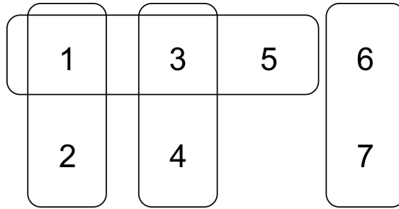
Figure 1 A hypergraph \{\{1, 2\}, \{3, 4\}, \{1, 3, 5\}, \{6, 7\}\}
