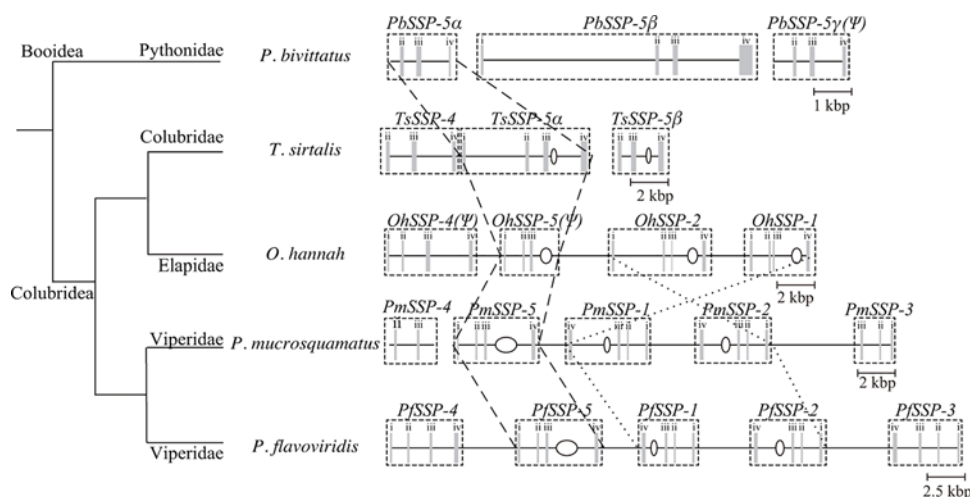
Figure 4. The relationship between the phylogenetic clade of snakes and the schematic structure of the configuration of the genes encoding SSPs
