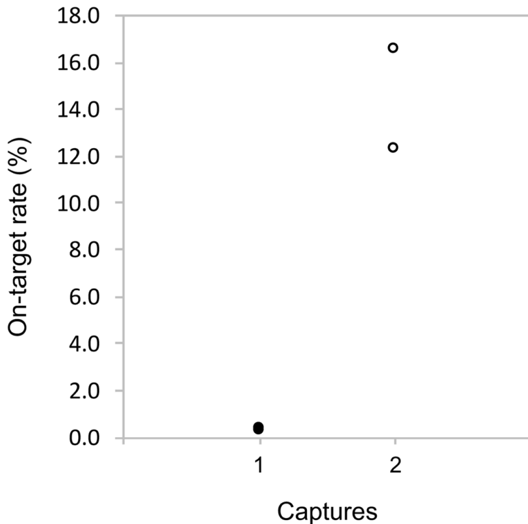
Fig 4. On-target rates depending on the number of captures. The formula to calculate the on-target rate is the same as in Fig 3.
