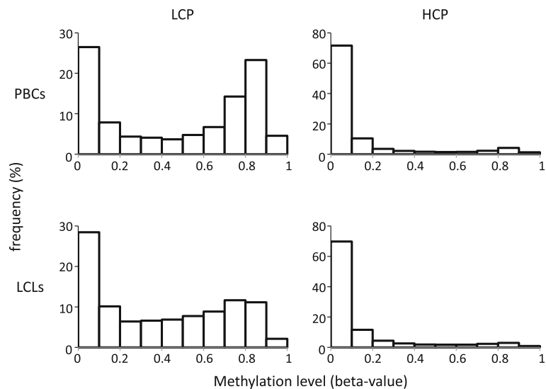
Fig. 5 Distribution of the methylation levels of the sites in the LCPs and HCPs. The frequency in the LCLs and PBCs are shown separately
