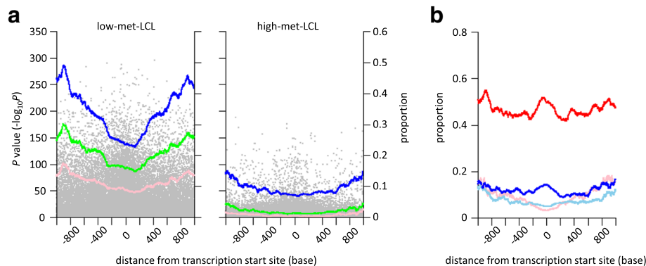
Fig. 3 Distribution of the differences in methylation levels between LCLs and PBLs in terms of TSS. a P values were plotted against the distance from the nearest TSS (gray dots). The proportion of the sites with P values ( -\log_{10}P ) greater than 10 (blue dots), 25 (green dots), and 50 (pink dots) in a window size of \pm 50 bases were plotted. b The proportion of the sites with P values ( -\log_{10}P ) greater than 10 obtained from non-CGI and CGI sites in the low-met-LCL group (red and pink dots, respectively), and from non-CGI and CGI sites in the high-met-LCL group (blue and sky blue dots, respectively) in a window size of \pm 50 bases were plotted against TSS
