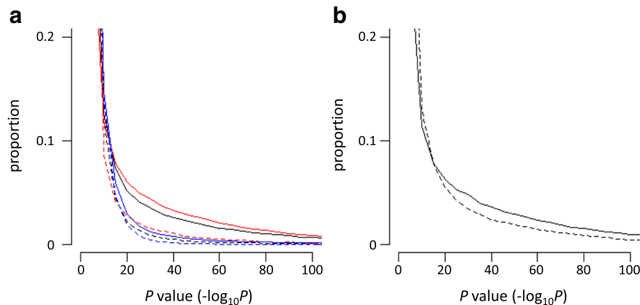
Fig. 2 Distribution of the differences in methylation levels between LCLs and PBLs in terms of CGI. a The proportion of P values obtained from non-CGI and CGI sites in all samples (black solid and dashed lines, respectively), non-CGI and CGI sites in the low-met-LCL group (red solid and dashed lines, respectively), and non-CGI and CGI sites in the high-met-LCL group (blue solid and dashed lines, respectively) are indicated. b The proportion of P values obtained from the non-shore and shore sites (solid and dashed lines, respectively) in the non-CGI sites of the low-met-LCL group are indicated
