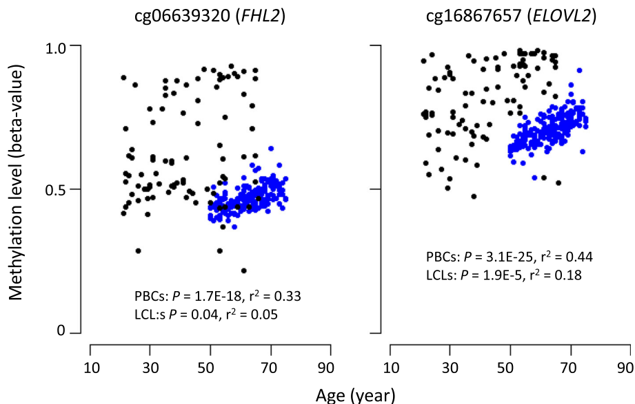
Fig. 6 Regression analyses of the methylation levels and chronological age at the FHL2 and ELOVL2 loci. The methylation levels in the LCLs (black dots) and PBCs (blue dots) were plotted against the age of the donors at the time of providing the specimens. The P values and r 2 were obtained by correcting for sex
