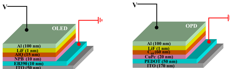
Fig. 6. Schematic illustration of the OPD (left) and OLED (right) structure [59] .
