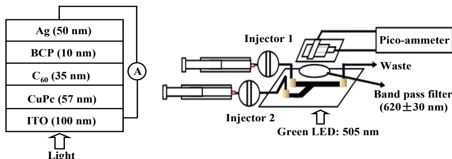
Fig. 4. Structure of the OPD and the schematic flow diagram of the fluorescence detection system [57] .
