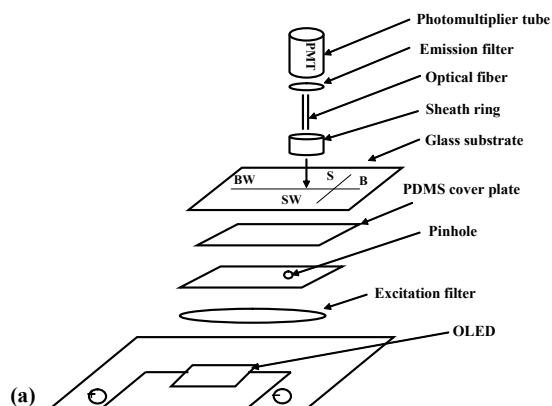
Fig. 1 Optical set-up of OLED induced fluorescence detection system: (a) detailed arrangement of each component, (b) side view of the structure with a coaxial optical fiber, and (c) side view of the structure with a perpendicular optical fiber [48] .
