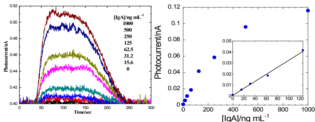
Fig. 5. Immunoassay of IgA using the OPD as an optical detector for fluorescence. (a) Fluorescence response of OPD as photocurrent, when the Amplex Red solution was introduced into the microchip, where the sandwich immunoreaction was carried out. (b) Calibration curve for IgA by plotting the photocurrent of OPD, which was the average for the time period from 70 s to 120 s in the plateau region of the response signal, against the concentration of IgA [57] .
