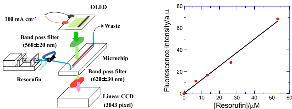
Fig. 3 Fluorescence detection system and calibration curve for IgA [56] .
