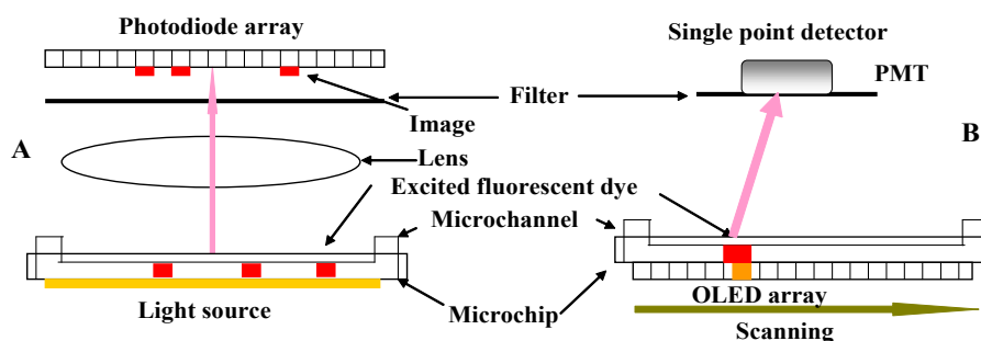
Fig. 2. A schematic diagram of the imaging mechanisms of CCD system and current work. The rectangles in yellow represent the lit OLED [55] .
