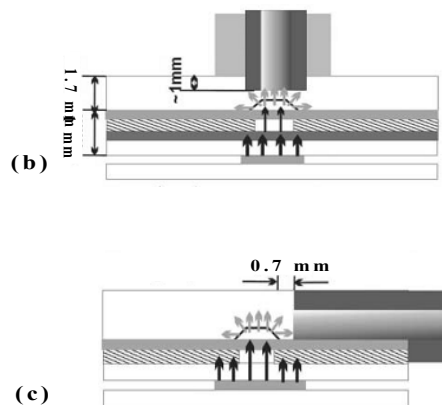
Fig. 1 Optical set-up of OLED induced fluorescence detection system: (a) detailed arrangement of each component, (b) side view of the structure with a coaxial optical fiber, and (c) side view of the structure with a perpendicular optical fiber [48] .
