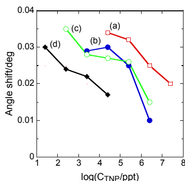
Fig. 28 Relationship between angle shift and concentration of TNP in the incubation solution. Concentration of TNP-KLH conjugate and 2 nd antibody in the incubation solution: (a) 100/25 ppm, (b) 150/25 ppm, (c) 150/35 ppm and (d) 200/35 ppm, respectively. The 1 st antibody was immobilized on the sensor chip by injecting 100 \mu L of a 100 ppm solution, volume of the incubation solution: 100 \mu L, carrier solution: phosphate buffer, pH 7.2, flow rate 20 \mu L min -1 .
