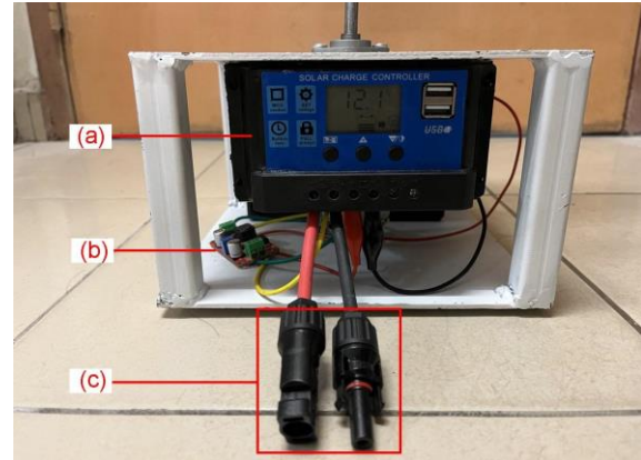
Fig. 7. Front view of frame and components. (a) PWM Battery Charge Controller; (b) DC-DC Boost Power Module; (c) MC4 connectors for solar panel.
