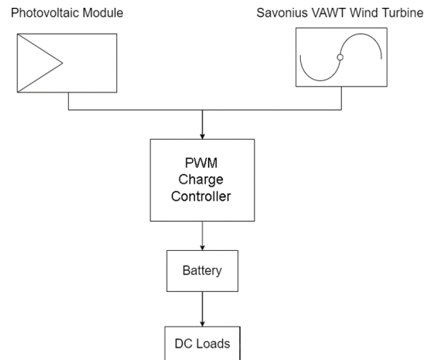
Fig. 1. Components used within hybrid renewable energy generation system.
