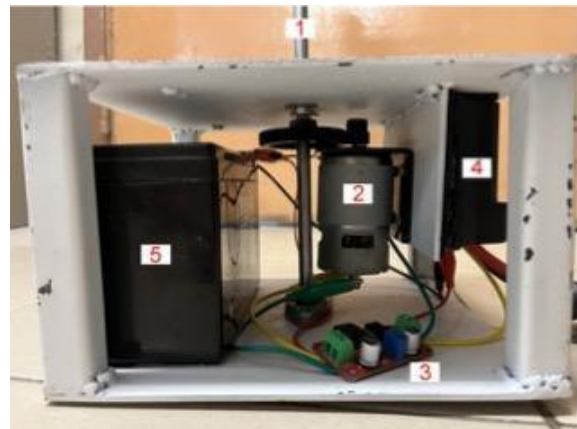
Fig. 8. Side view of frame and components. (1) Shaft connected to VAWT and gears; (2) DC motor; (3) DC-DC Boost Power Module; (4) PWM BCC; (5) 12 V Battery.
