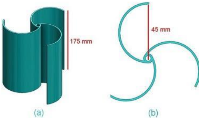
Fig. 3. Three-bladed VAWT composition. (a) Isometric view; (b) Top view
