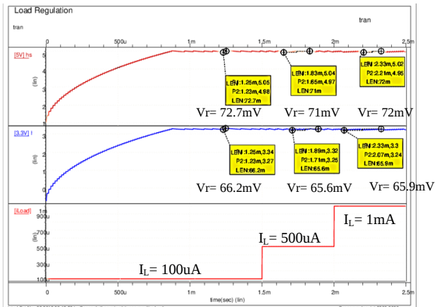
Fig.14. Boost Convert Load Regulation
