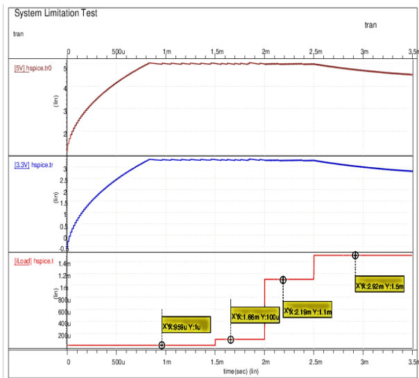
Fig.15. System Limitation Test
