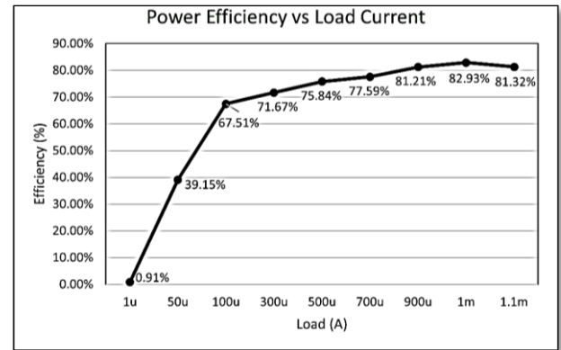
Fig 16. System Limitation Test
