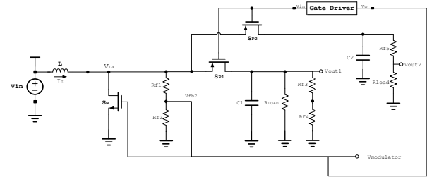
Fig. 9 Power Stage
