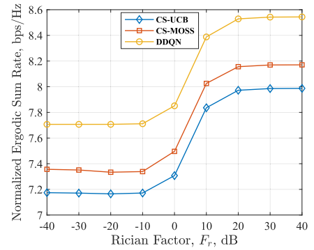
FIGURE 11. Tracking the maximum deployment performance of the DDQN agent vs cost-subsidized MAB for varying levels of LOS component presence.
