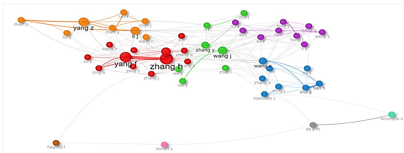
Fig. 16: collaboration network.
