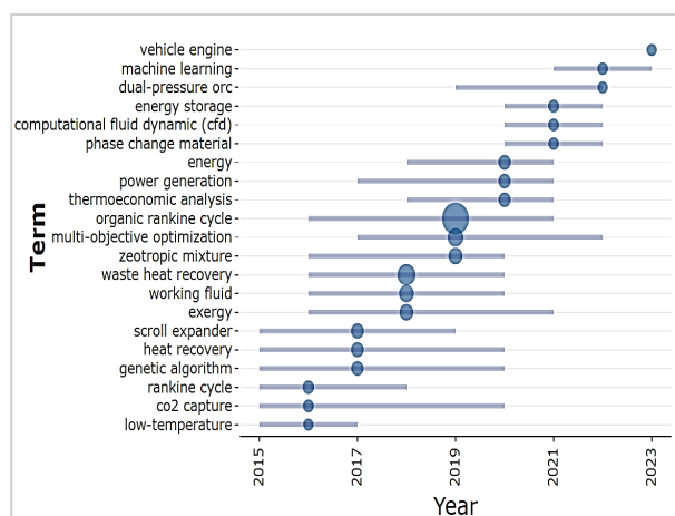
Fig. 18: Trend topics.
