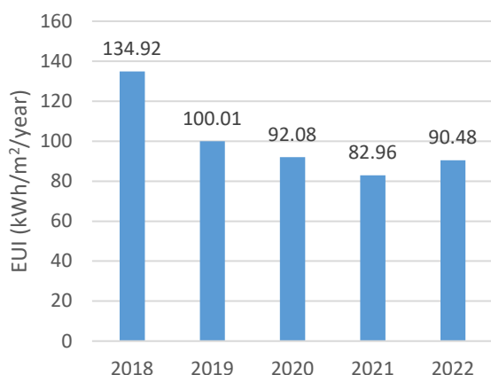
Fig. 9: Energy Use Intensity (Electricity) in \text{kWh}/\text{m}^2/\text{year} from 2018-2022
