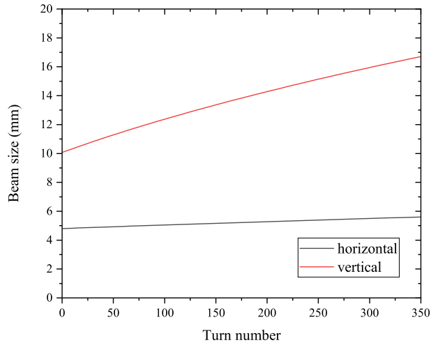
Fig. 3. Beam size as a function of turn number.
