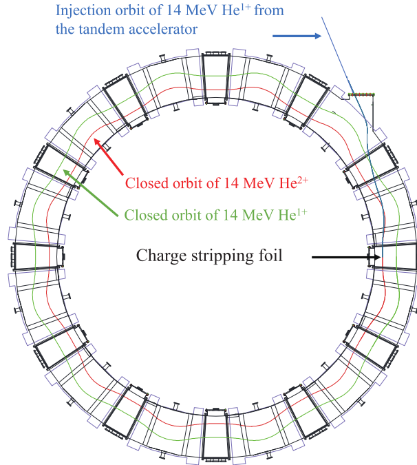
Fig. 2. Injection orbit of \text{He}^{1+} (blue line), closed orbit of \text{He}^{1+} (green line), and closed orbit of \text{He}^{2+} (red line). The charge-stripping foil is installed at the intersection of the injection orbit and the closed orbit of \text{He}^{2+} .
