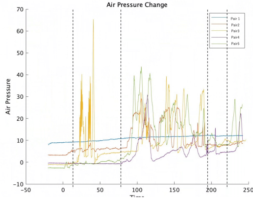
Fig.8: Air pressure change during watching VID_408, a video of an astronaut landing on Earth from space.
