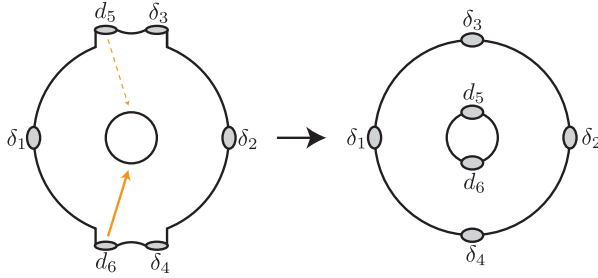
(b) Rearrangement of the boundary components.
