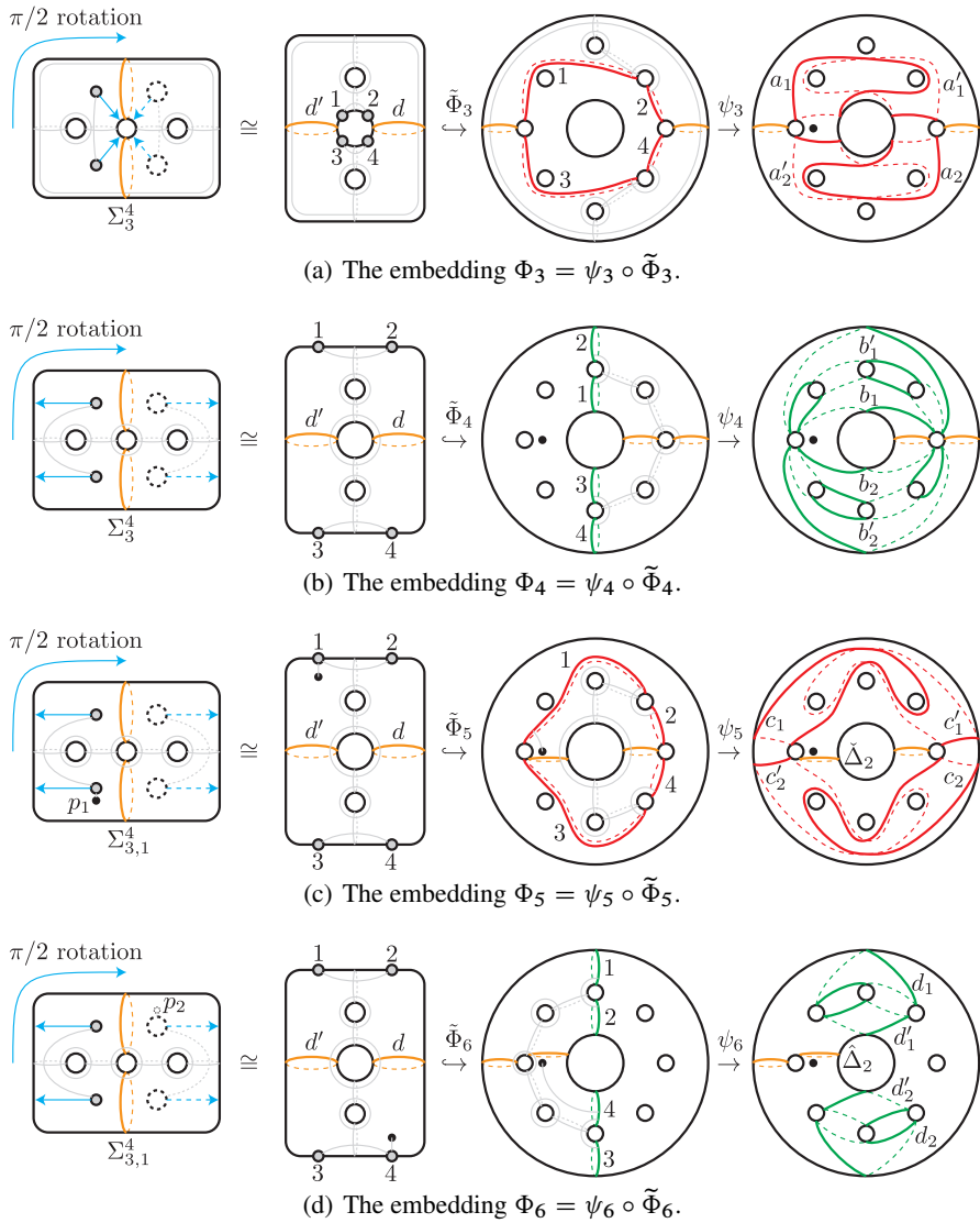
Fig. 20. The embeddings.
