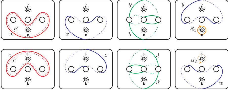
Fig. 14. A lift of the genus-3 relation to \text{Mod}(\Sigma_{3,2}^4) .
