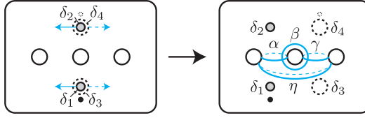
Fig. 18. Sliding the boundary components and the curves for the conjugation.
