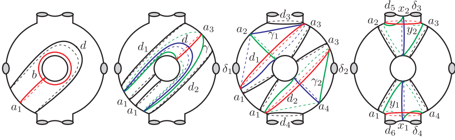
(a) The 2-chain relation and lantern relations.
