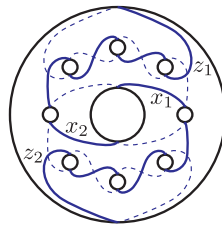
Fig. 25. The bounding quadruple.
