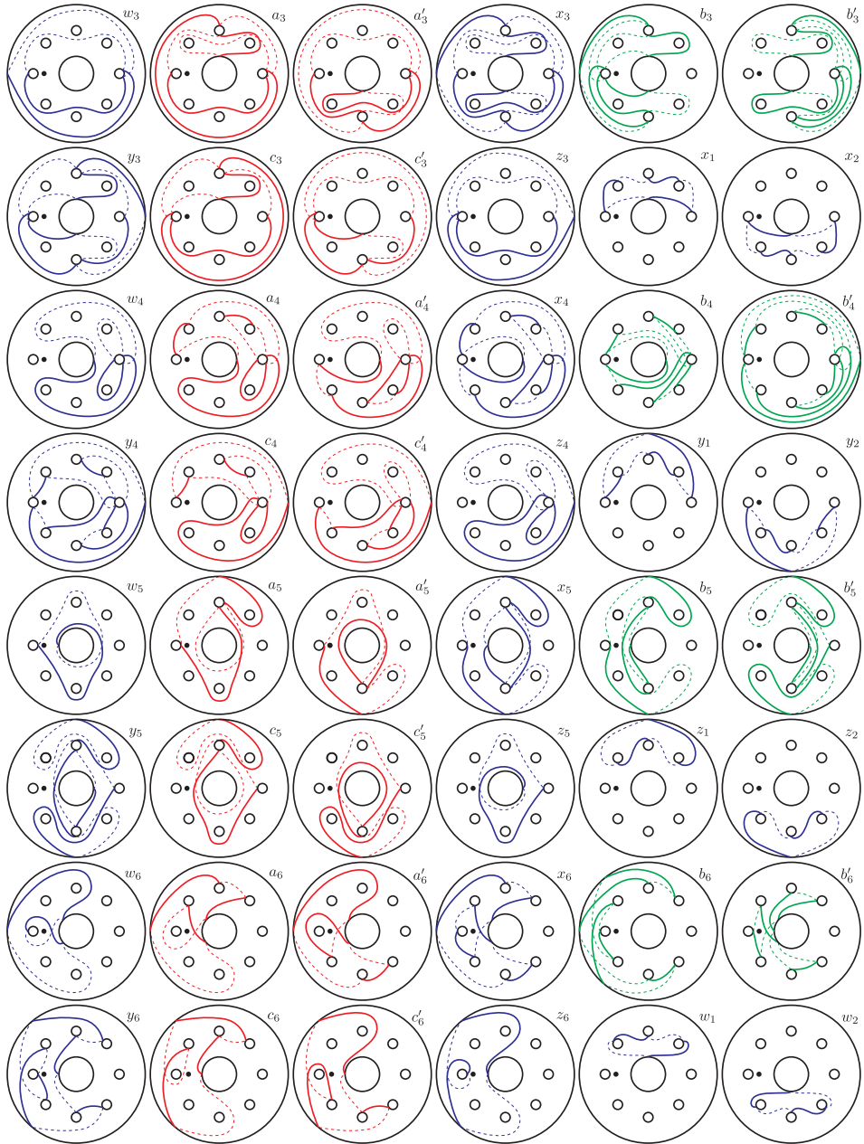
Fig. 23. Vanishing cycles of the genus-9 Lefschetz fibration with signature zero.
