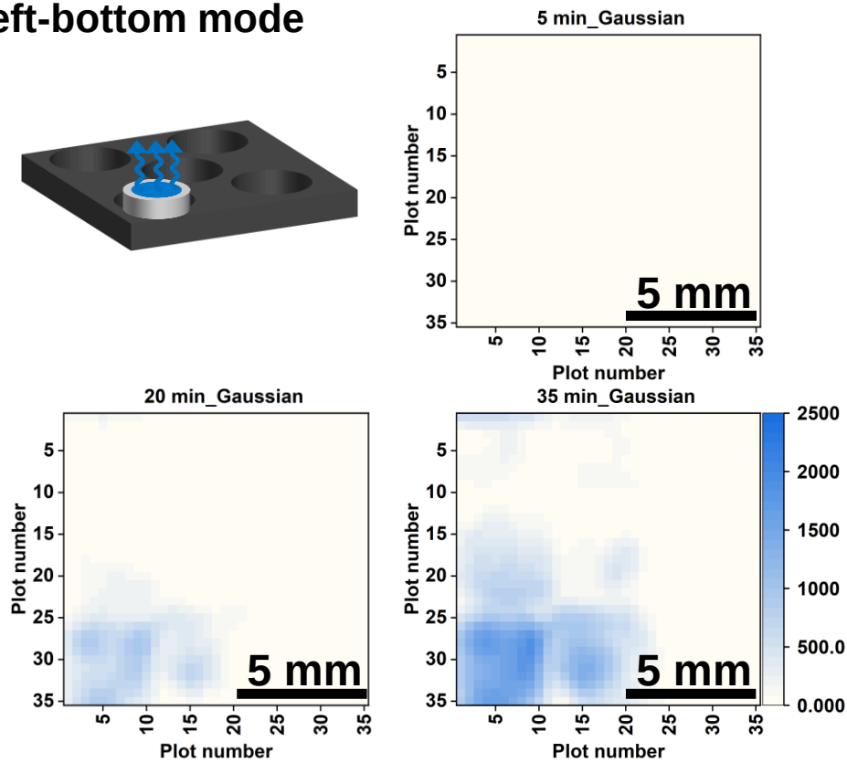
Fig. 4. 8. The visualization of benzaldehyde odor at 5 min, 20 min and 35 min when the odor source was placed at the left-bottom corner.
