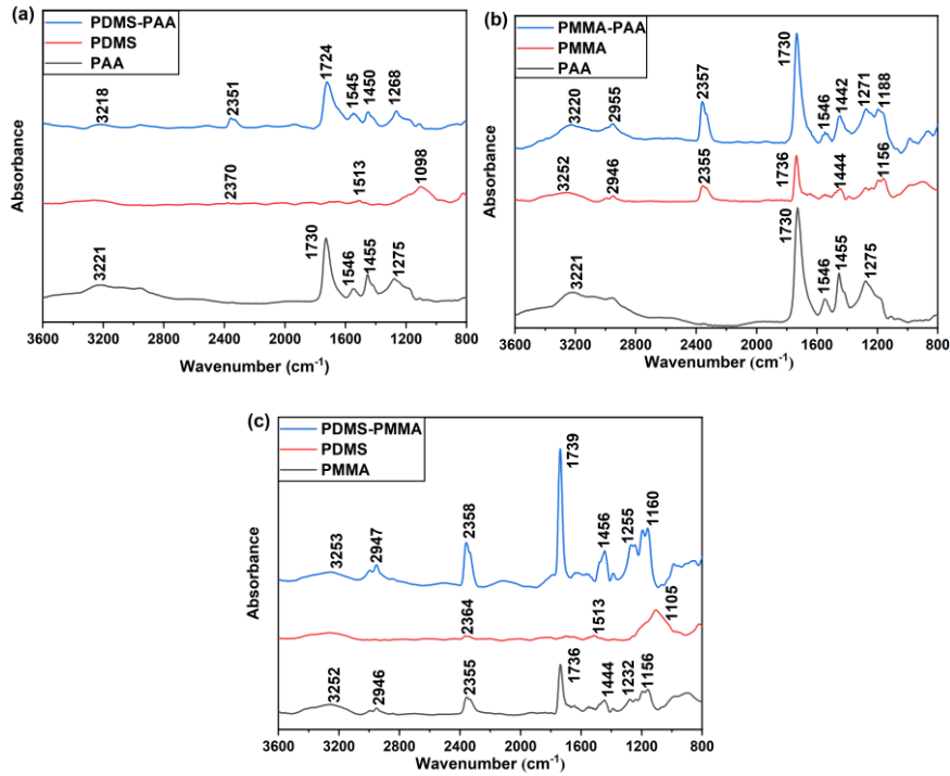
Fig. 3. 4. FT-IR spectra in the range 800-3600 cm -1 of SERS gas sensor coated by (a) PDMS-PAA, (b) PMMA-PAA and (c) PDMS-PMMA polymer film.
