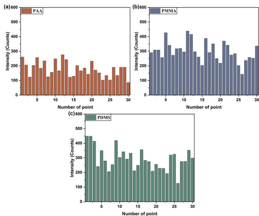
Fig. S3. 7. SERS intensities at 1175 cm -1 of random 30 points obtained by using (a) PAA, (b) PMMA and (c) PDMS coated sensors for anethole gas detection.
