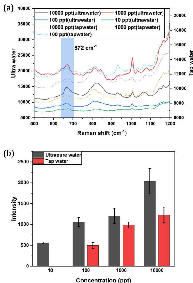
Fig. 2. 9. Comparison of (a) SERS spectra and (b) SERS intensity at 672 cm -1 of various geosmin solutions diluted in tap water and ultrapure water.
