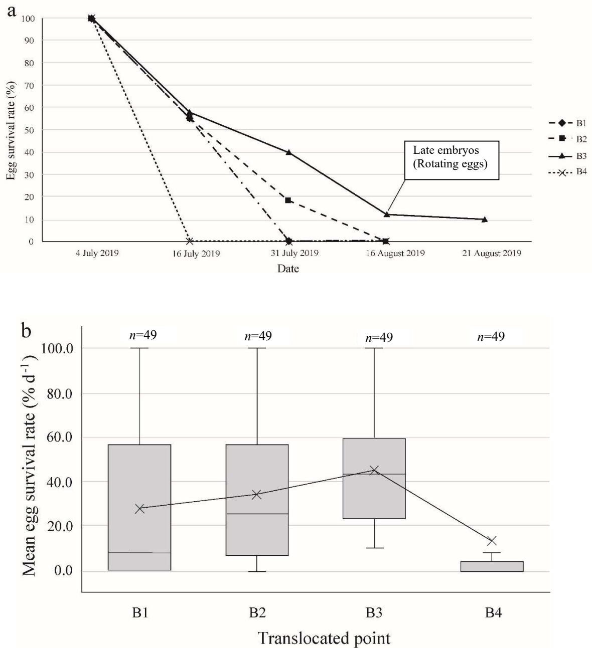
Figure 4.4 a) Changes in the survival rate of translocated eggs at transect B over the study period. b) Comparison of mean egg survival rates per day at transect B over the study period.
