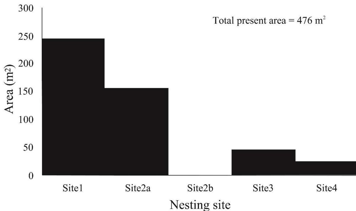
Figure 5.6 Estimated present suitable spawning area in Tsuyazaki, Fukuoka, Japan.
