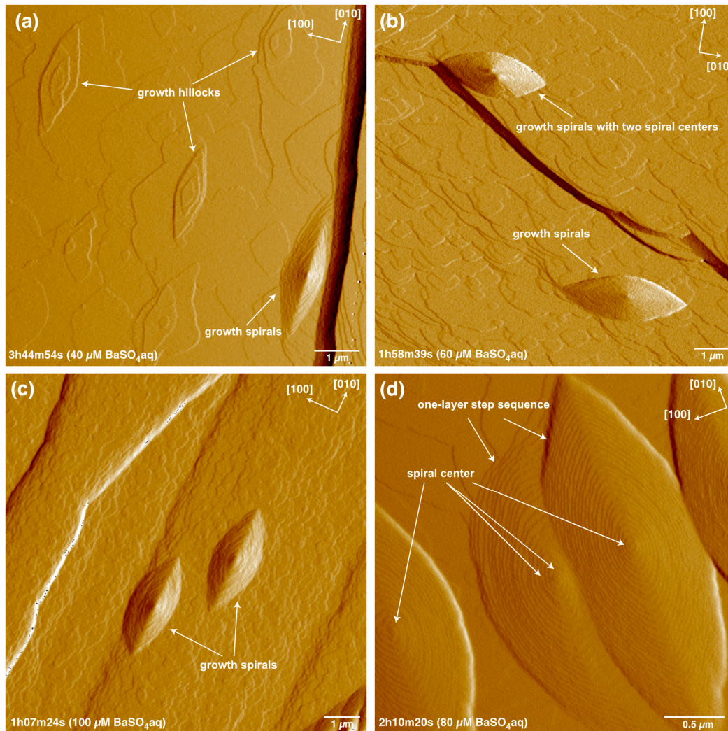
Figure 4. (a–c) CMAFM deflection images of a (001) surface in 40 \mu\text{M} , 60 \mu\text{M} , and 100 \mu\text{M} \text{BaSO}_4 solutions at 30 ^{\circ}\text{C} , respectively, showing the growth spirals that formed from screw dislocations. The growth hillocks that likely formed from edge dislocations are also shown in (a). (d) CMAFM deflection image of a (001) surface in an 80 \mu\text{M} \text{BaSO}_4 solution at 30 ^{\circ}\text{C} showing growth spirals with a one-layer step sequence and regular step spacing.
