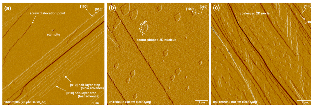
Figure 1. (a–c) CMAFM deflection images of a (001) surface in 20 \mu\text{M} , 40 \mu\text{M} , and 100 \mu\text{M} \text{BaSO}_4 solutions at 30 ^{\circ}\text{C} , respectively. In (b), sector-shaped 2D nuclei formed sporadically, while in (c) these nuclei formed rapidly and coalesced.
