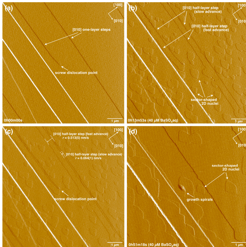
Figure 2. (a), (b), and (d) Sequential CMAFM deflection images of a (001) surface in a 40 \mu\text{M} \text{BaSO}_4 solution at 30 ^{\circ}\text{C} after 0 min, 14 min, and 51 min, respectively; each one-layer [010] step (step height = 7.2 \text{\AA} ) begins to split into two half-layer steps (step height = 3.6 \text{\AA} ) with different advance rates. Sector-shaped 2D nuclei were randomly formed, independent of the microtopography. In (d), the birth of a growth spirals that formed from a screw dislocation point is shown. (c) A comparison of (a) and (b), which are overlapped. The splitting process and advance rates of the steps are clearly demonstrated.
