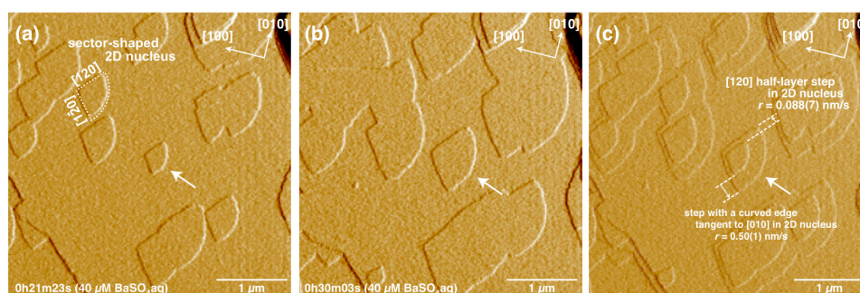
Figure 5. (a) and (b) Sequential CMAFM deflection images of a (001) surface in a 40 \mu\text{M} BaSO 4 solution at 30 °C after 21 min and 30 min, respectively; (c) a comparison of (a) and (b), which are overlapped. The lateral spreading process and step advance rates of the 2D nuclei are clearly demonstrated. See Figure 6 for the growth of a 2D nucleus that is indicated by the white arrows.
