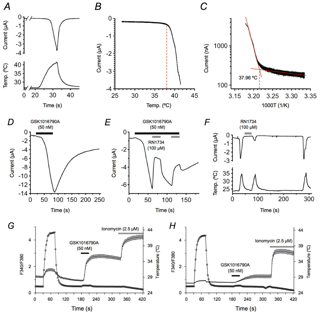
Figure 2. AmTRPV4 is a thermosensitive TRP channel that activates near alligator TSD temperature range. (A) A representative trace of the current (upper) activated in response to corresponding changes in both solution temperature (lower) in the Xenopus oocytes expressing AmTRPV4 using a two-electrode voltage-clamp method. (B) A representative temperature-response profile for AmTRPV4 activation by heat. (C) A representative Arrhenius plot for heat-induced AmTRPV4 activation. The average threshold for activation was 37.30 \pm 0.54 °C; n = 17 . (D) A representative trace of the AmTRPV4 current in the oocyte activated by a TRPV4 agonist (GSK1016790A indicated in a black bar); n = 4 . (E) A representative trace of AmTRPV4 current in the oocyte activated by administration of a specific TRPV4 agonist (GSK1016790A indicated by a black bar) and subsequently inhibited by TRPV4 specific antagonist (RN1734 indicated by a gray bar); n = 4 . (F) A representative current trace of AmTRPV4 expressing oocyte activated by heat stimulus and subsequently inhibited by a specific TRPV4 antagonist (RN1734 indicated by a gray bar); n = 4 . (G) A representative averaged changes of [Ca^{2+}]_i in AmTRPV4-expressing HEK293 cells ( n = 75 ) under both heat and chemical stimulation. [Ca^{2+}]_i changes in AmTRPV4-expressing cells (indicated as an average trace \pm SE; left y-axis) were observed along with temperatures (indicated by open circle trace; right y-axis). Applications of a TRPV4 agonist (GSK1016790A) and ionomycin are shown with a black and gray bars, respectively. (H) Representative [Ca^{2+}]_i and temperature changes in mock transfected HEK293 cells ( n = 36 ).
